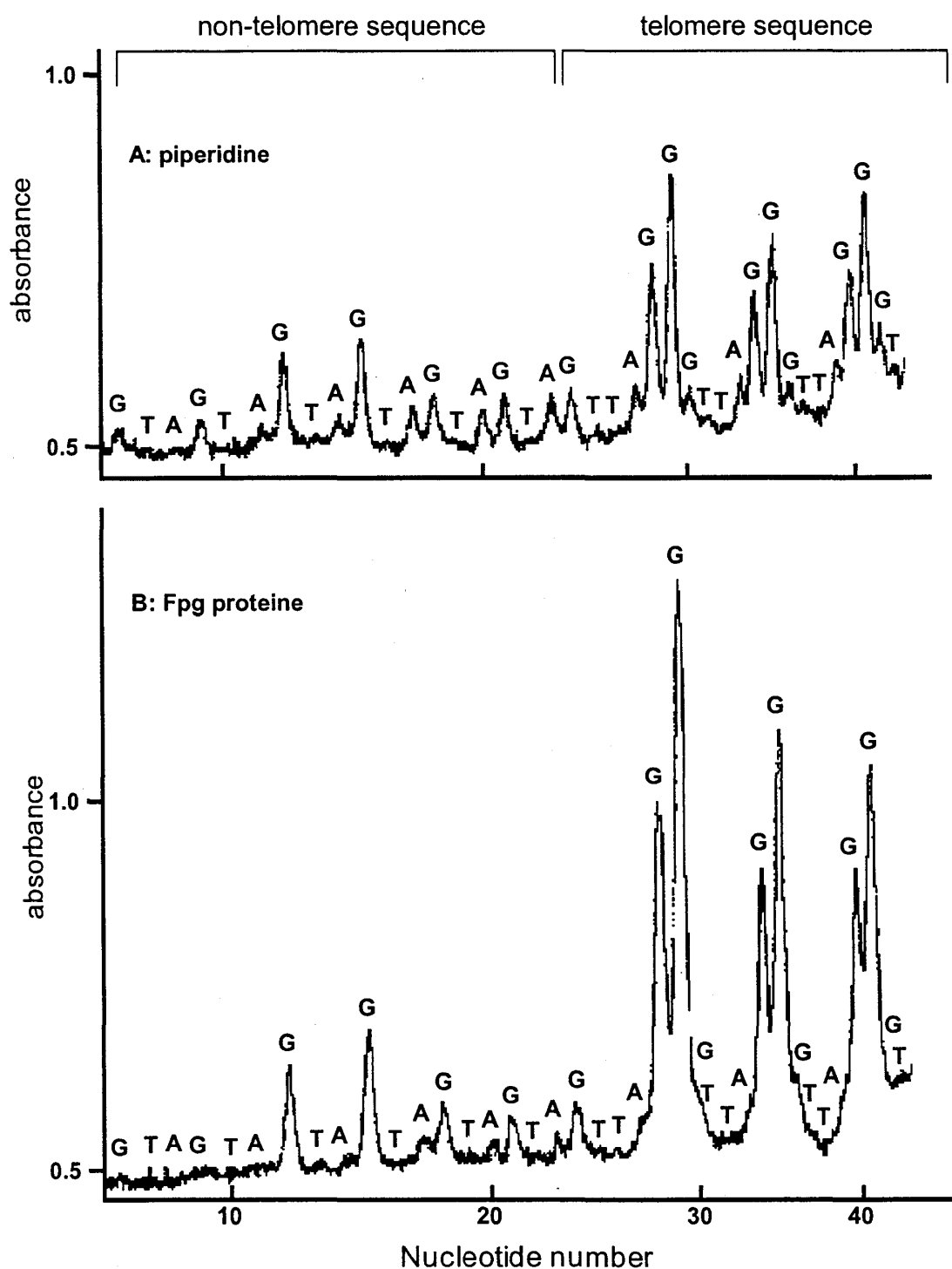
図2. リボフラビン存在下UVAによるDNA損傷の塩基配列特異性 The ^{32}\text{P} 5' end-labeled 48-base pair fragment (5'-(TAGTAG) _4 (TTAGGG) _4 -3') was exposed to 2 J/cm ^2 UVA light (365 nm) with 20 \mu\text{M} riboflavin in 100 \mu\text{l} of 10 mM sodium phosphate buffer (pH 7.8) containing 5 \mu\text{M} DTPA. After piperidine (A) or Fpg protein (B) treatment, DNA fragments were electrophoresed on a 12% polyacrylamide/8 M urea gel using a DNA-sequencing system and the autoradiogram was obtained by exposing X-ray film to the gel. The relative amounts of oligonucleotides produced were measured using a laser densitometer. The cleavage sites of the treated DNA were determined by direct comparison with the same DNA fragment after undergoing DNA sequencing reactions according to the Maxam Gilbert procedure. The horizontal axis shows the nucleotide number.
