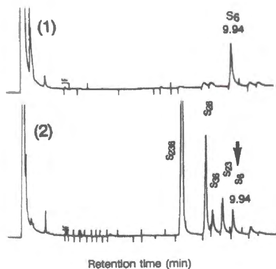
Figure 3-4. GLC patterns of alditol acetates from (1) 6- O -ethylcellulose and (2) commercial O -ethylcellulose (DS 2.3).
