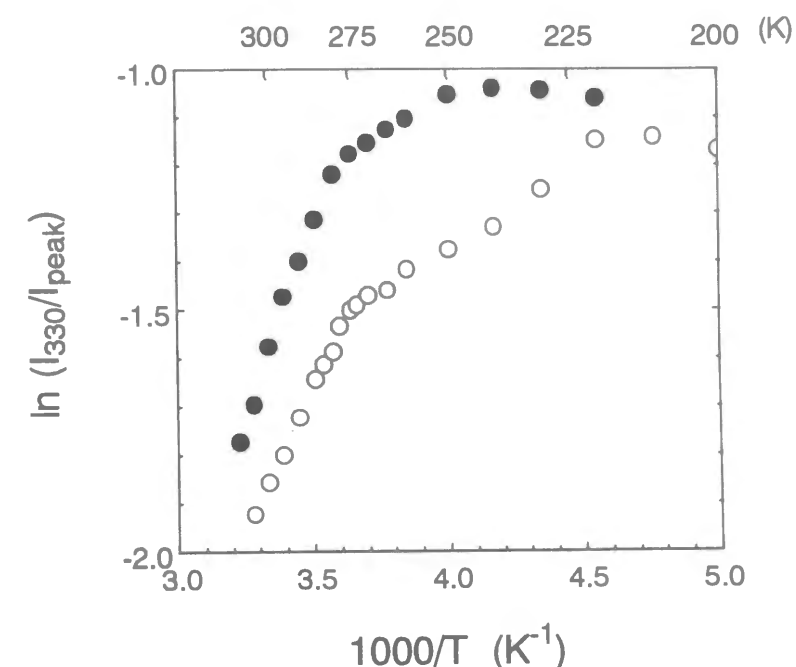
Figure 7-5. Temperature dependence of I_{330}/I_{\text{peak}} for 2.3% 2,3-BC in THF: (○) cooling from 305 to 200 K; (●) heating from 200 to 310 K. All the I_{330}/I_{\text{peak}} values are the equilibrium ones.
