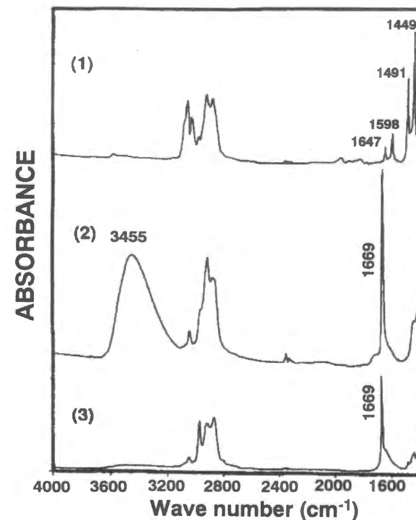
Figure 3-1. IR spectra of (1) 2,3-di- O -allyl-6- O -tritylcellulose, (2) 2,3-di- O -(1-propenyl)cellulose, and (3) 6- O -ethyl-2,3-di- O -(1-propenyl)cellulose.
