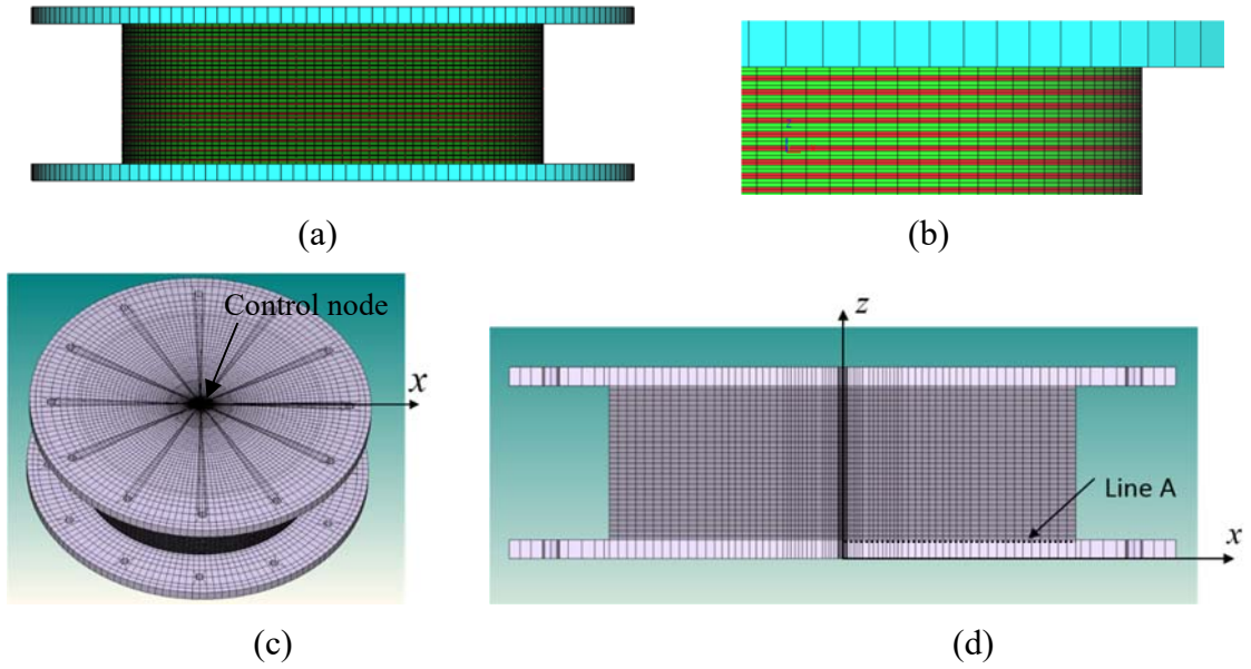
Figure 1. FE-mesh of a rubber bearing model; (a) side view, (b) close view of upper left, (c) diagonal view, (d) section in the xz -plane.
