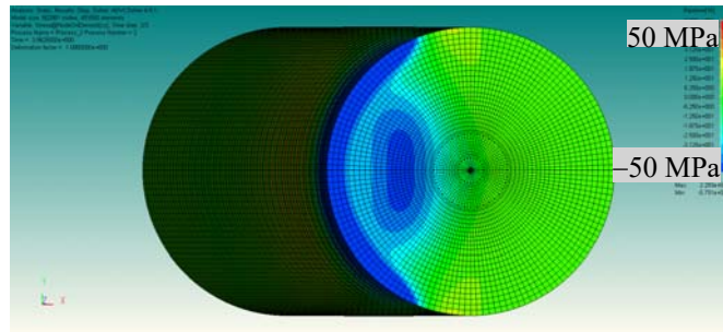
Figure 8. Vertical stress on the upper surface of the top rubber sheet at maximum deformation.
