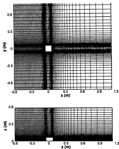
Fig. 5 calculation mesh (B-type)
