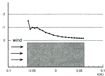
Fig. 14 Pressure distribution on the center line of roof surface (B-type)
