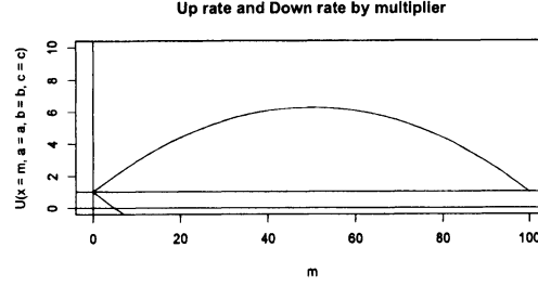
Figure 11: Cushion change rate by multiplier
