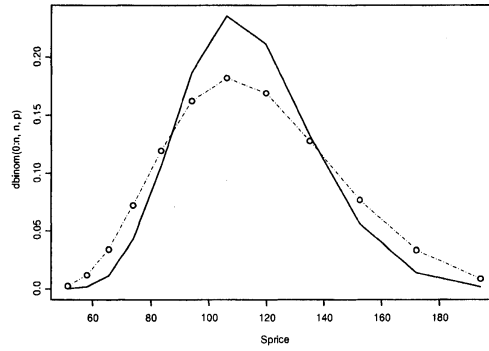
Figure 8: Binomial vs Bushy tree distribution
