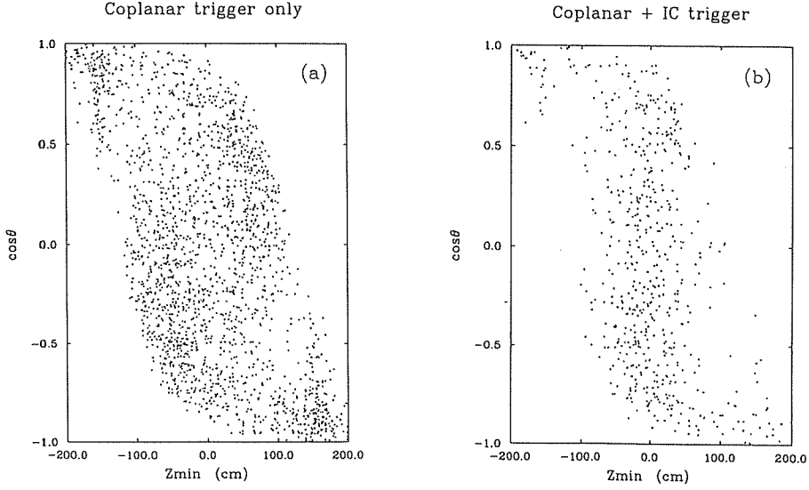
Figure 6 Scatter plots in \cos \theta and Z_{\min} of the charged tracks for the events accepted by the coplanar trigger without the Z-trigger (a) and for the events accepted by the coplanar trigger with the Z-trigger (b).
