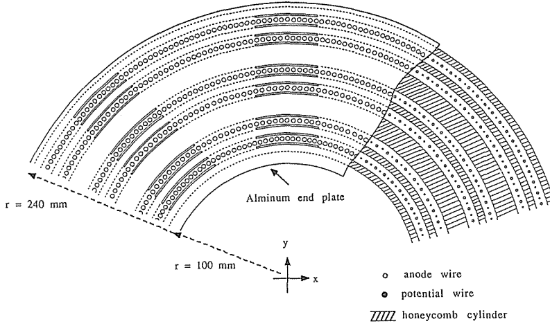
Figure 2 Part of the r - \theta view of the inner chamber endplate. The left half side of the figure shows the aluminum endplate. Here, the circles are the holes for supporting the wires. The right half side shows the chamber structure, where the circles and the dashed area indicate the wires and the honeycomb cylinder, respectively.
