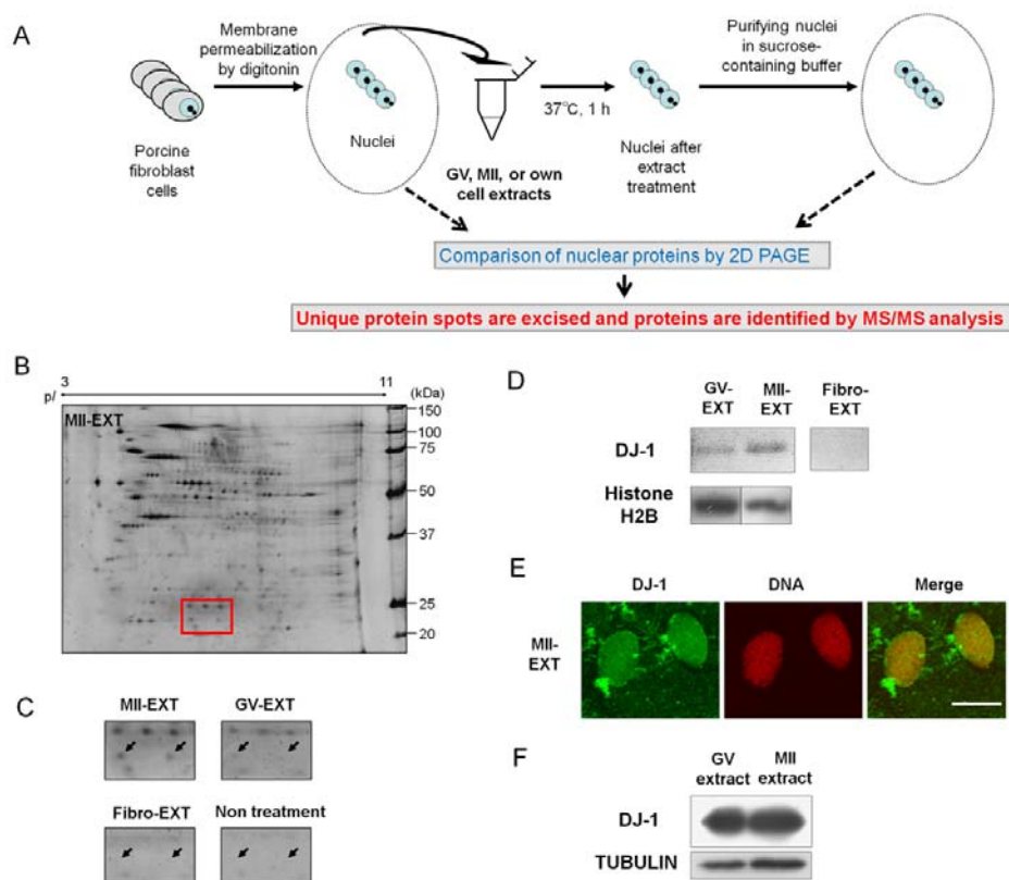
Fig. 1. Identification of protein DJ-1 as a candidate reprogramming factor present in the MII oocytes.
