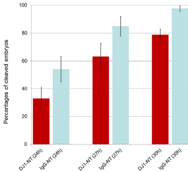
Fig. S5. Timing of first cleavage was compared between NT embryos injected with DJ-1 antibody (DJ1-NT) and those with IgG (IgG-NT). The y axis represents ratios of cleaved embryos at different times (24 h, 27 h, and 30 h) to total cleaved embryos at 48 h.
