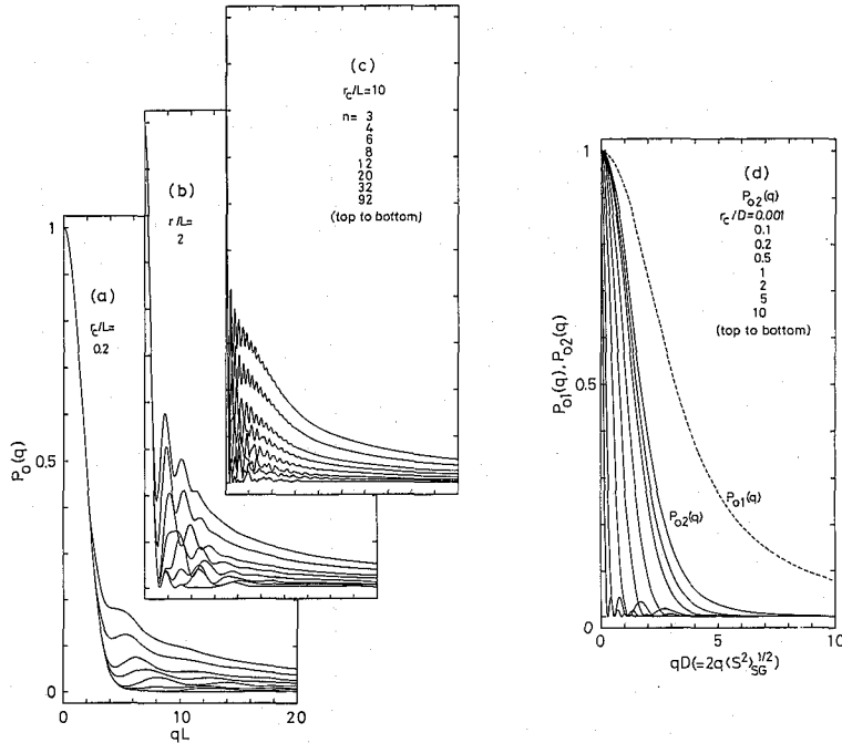
Figure 1(a)-(d). The particle scattering functions for the rodlike shell P_o(q) with (a) r_c/L = 0.2 , (b) r_c/L = 2 , and (c) r_c/L = 10 . The number of rods n is changed as 3, 4, 6, 8, 12, 20, 32, and 92 from the top to the bottom. (d) The particle scattering functions for the shell of Gaussian chains. The broken line represents the intrachain part P_{o1}(q) and the solid lines represent the interchain part P_{o2}(q) , the ratio r_c/2\langle S^2 \rangle_{SG}^{1/2} being 0.001, 0.1, 0.2, 0.5, 1, 2, 5, and 10 from the top to the bottom.
