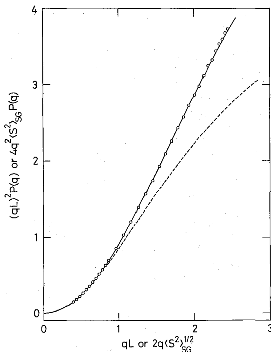
Figure 7. The results of the data fitting. The unfilled circles represent the data for poly (N-ethyl-2-vinylpyridinium hydroxide)- block -polystyrene in salt-free aqueous solution at 25°C. The solid line denotes the theoretical P(q) calculated for the rodlike-shell micelles with r_c = 10.7 nm and L = 95.7 nm, while the broken line for the Gaussian-shell micelles with the same values, r_c = 10.7 nm and D = 2\langle S^2 \rangle_{\text{SG}}^{1/2} = 95.7 nm.
