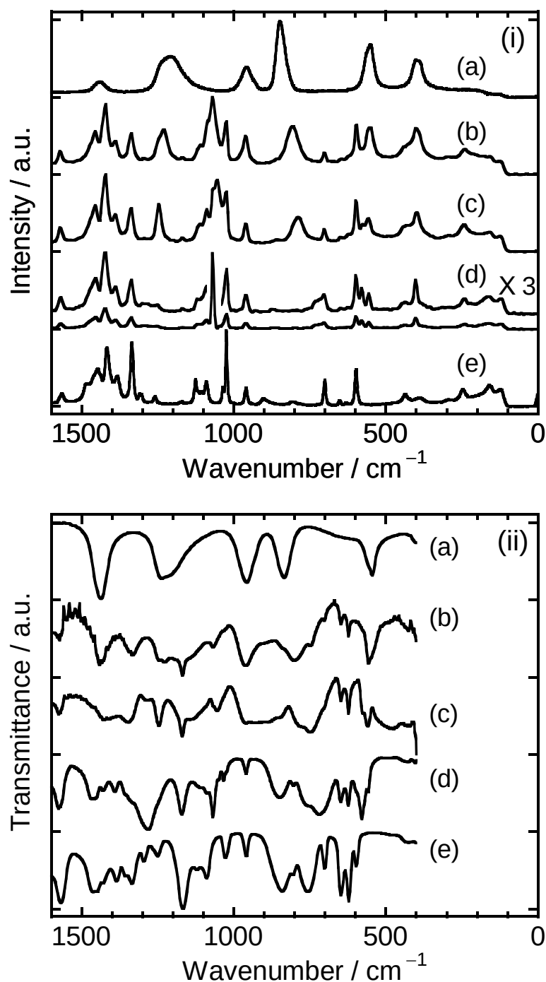
Figure 2. (i) Raman and (ii) IR spectra of (a) \text{HOSO}_2\text{F} (b) \text{EMIm}(\text{FO}_2\text{SOH})_2\text{O}_2\text{SOF} (c) \text{EMIm}(\text{FO}_2\text{SOH})\text{OSO}_2\text{F} , (d) \text{EMImSO}_3\text{F} (with the spectrum multiplied by 3 for clarity in the Raman spectrum), and (e) \text{EMImCl} .
