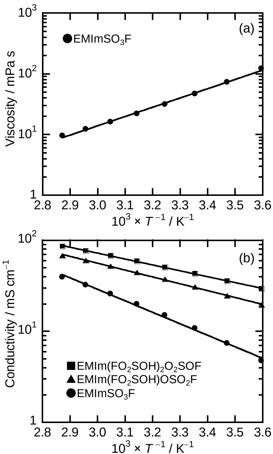
Figure 4. Arrhenius plots of (a) viscosity for EMImSO 3 F and (b) ionic conductivity for EMIm(FO 2 SOH) n O n SO 3-n F ( n = 0, 1 , and 2).
