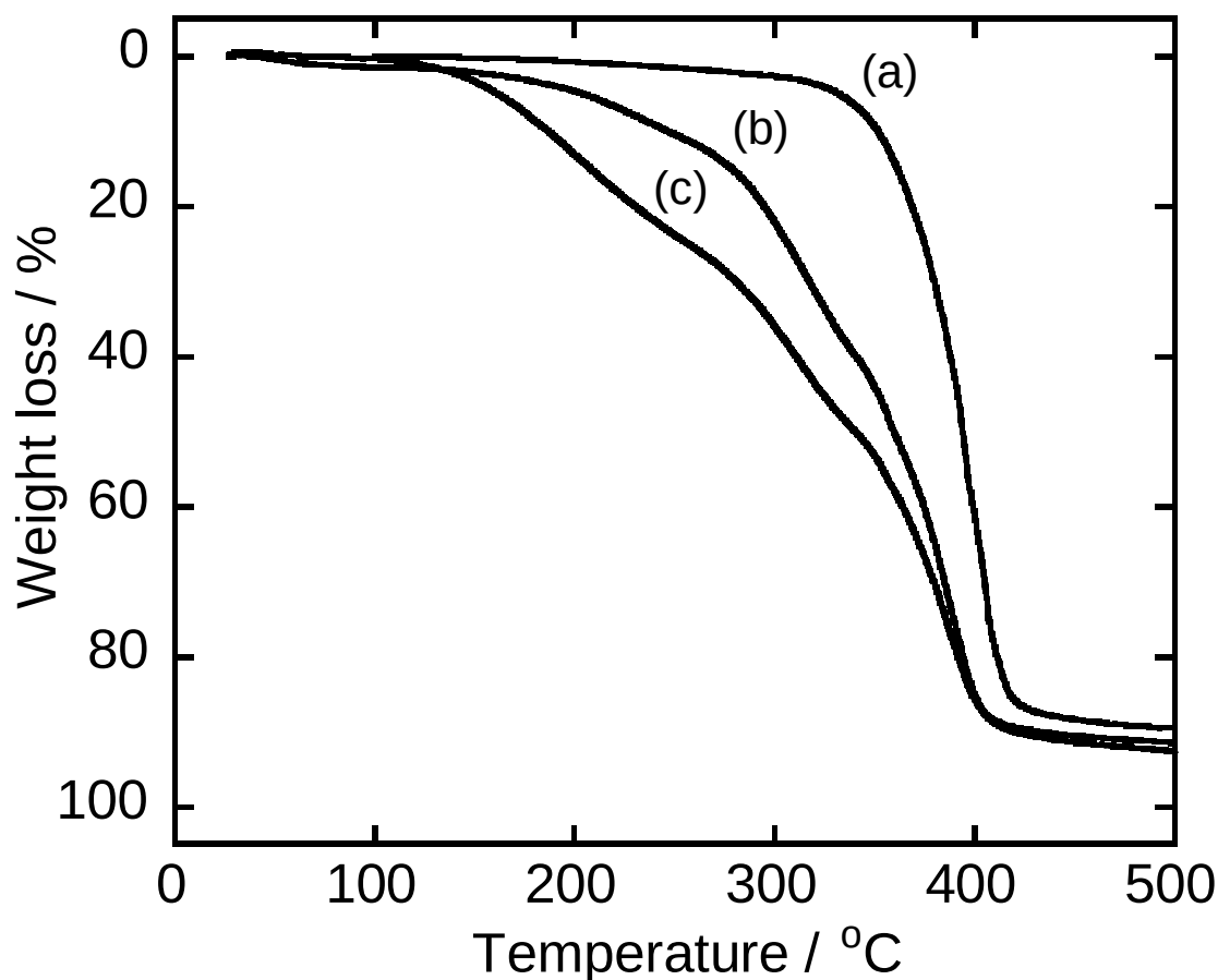
Figure 3. Thermogravimetric curves for EMIm(FO 2 SOH) n O n SO 3-n F ( n = 0, 1 , and 2 ); (a) EMImSO 3 F, (b) EMIm(FO 2 SOH)OSO 2 F, and (c) EMIm(FO 2 SOH) 2 O 2 SOF. Scan rate of 10^{\circ}\text{C min}^{-1} was used.
