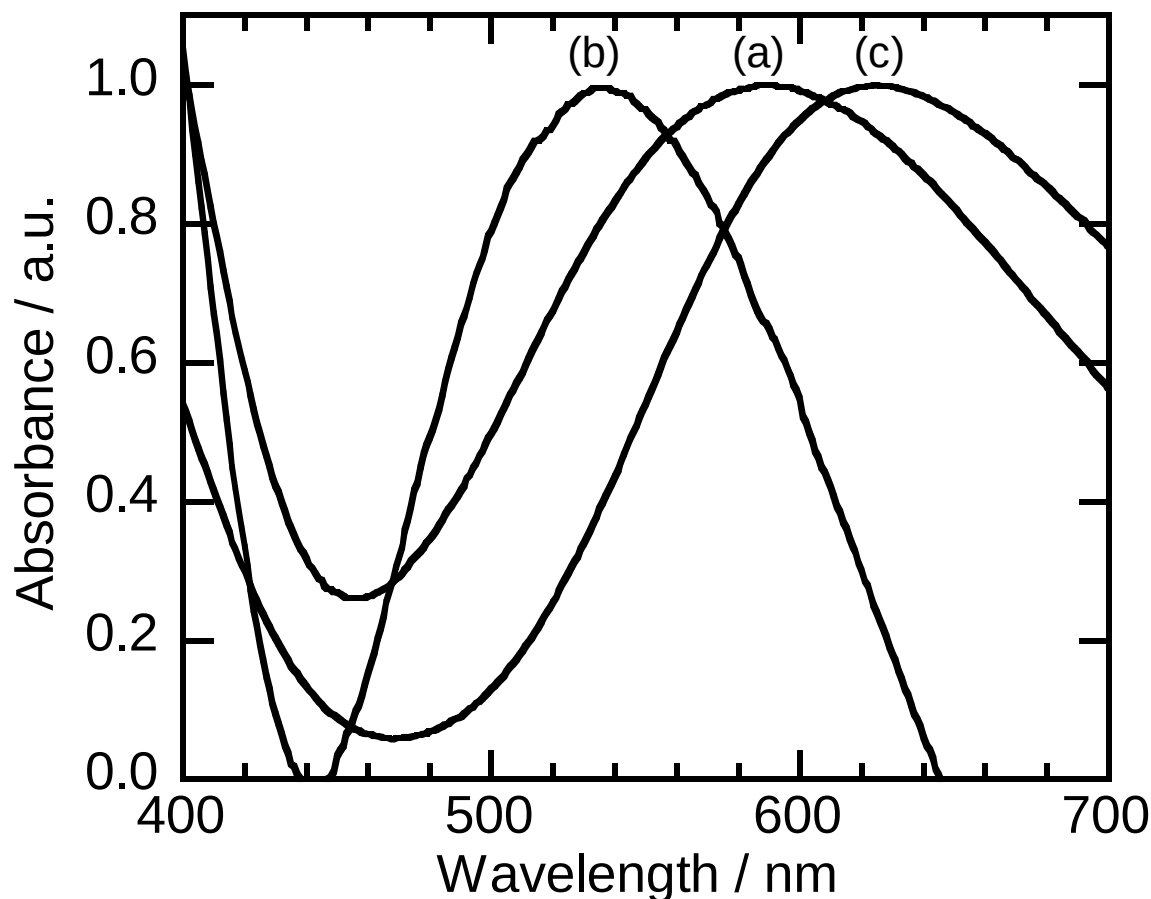
Figure 5. Visible absorption spectra of EMIm-based ILs containing 0.01 M of [\text{Cu}(\text{tmen})(\text{acac})][\text{BPh}_4] . (a) EMImSO 3 F, (b) EMImBF 4 , and (c) EMImPO 2 F 2 . For (b) EMImBF 4 and (c) EMImPO 2 F 2 , see ref. 13.
