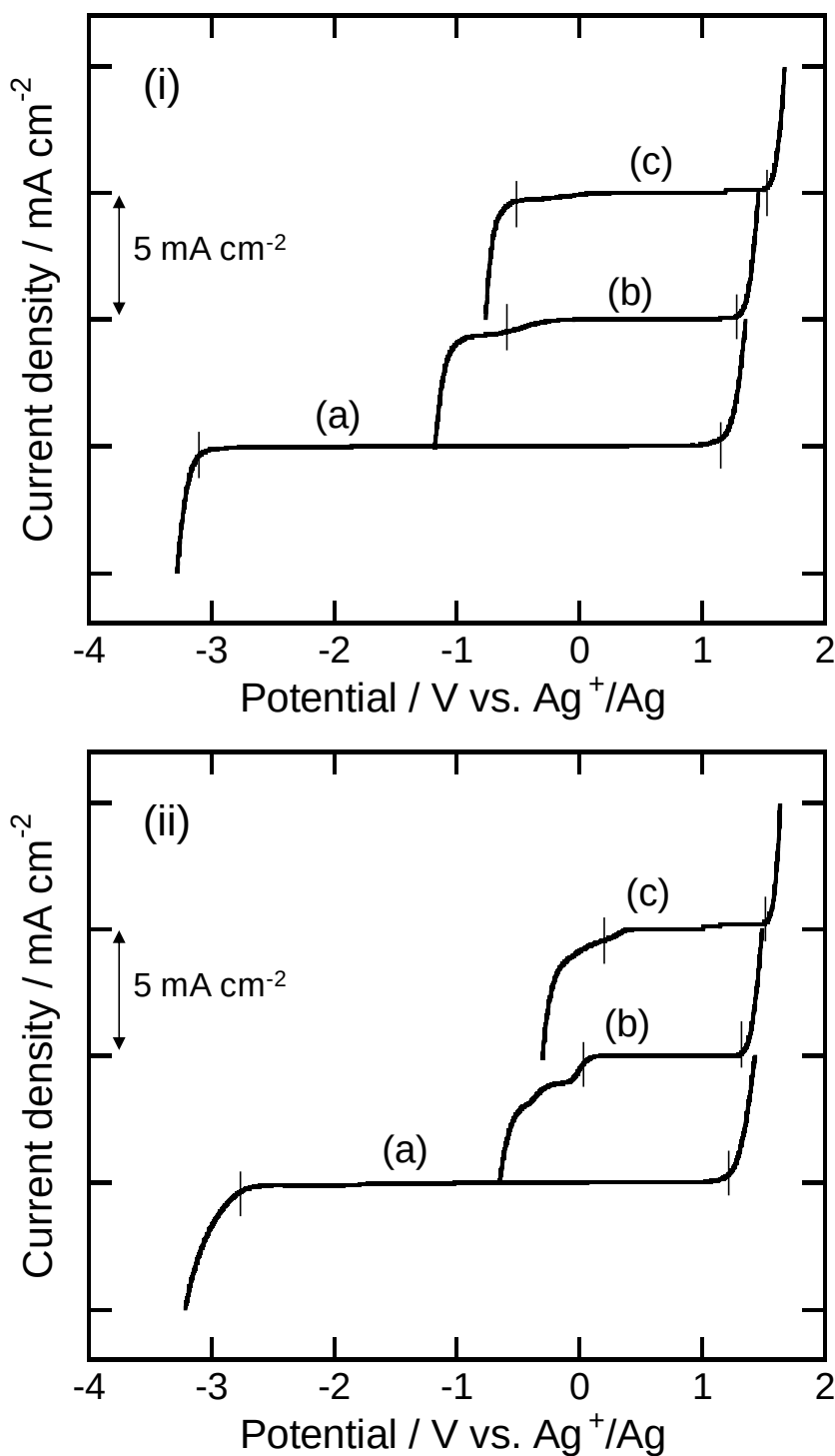
Figure 6. Linear sweep voltammograms of (i) glassy carbon and (ii) platinum electrodes in EMIIm(FO 2 SOH) n O n SO 3-n F ( n = 0, 1 , and 2 ); (a) EMIImSO 3 F, (b) EMIIm(FO 2 SOH)OSO 2 F, and (c) EMIIm(FO 2 SOH) 2 O 2 SOF. Vertical lines denote the anode and cathode limits determined as the potentials where the absolute values of the current densities exceed 0.5 mA cm -2 at the scan rate of 10 mV s -1 .
