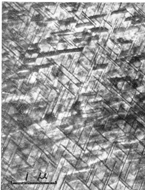
Photo. 51 Al-Ag-Zr alloy, W.Q., aged for 4 hrs at 200°C. ×20000
