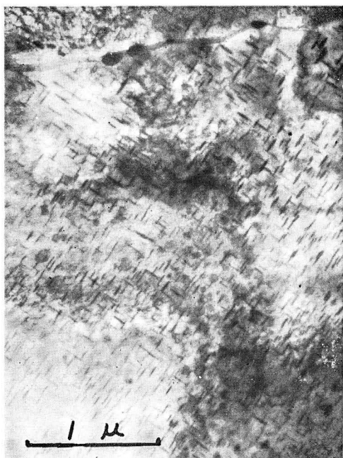
Photo. 35 Al-Cu-0.3% Be alloy, W.Q., 5.0% elong., aged for 1 day at 200°C. \times 25000
