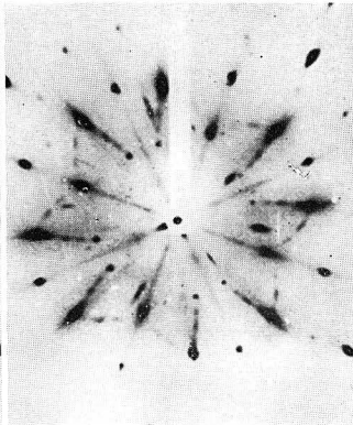
Photo. 14 Al-Cu-Ti alloy W.Q., elong. 2% and aged 1 day at 150°C.
