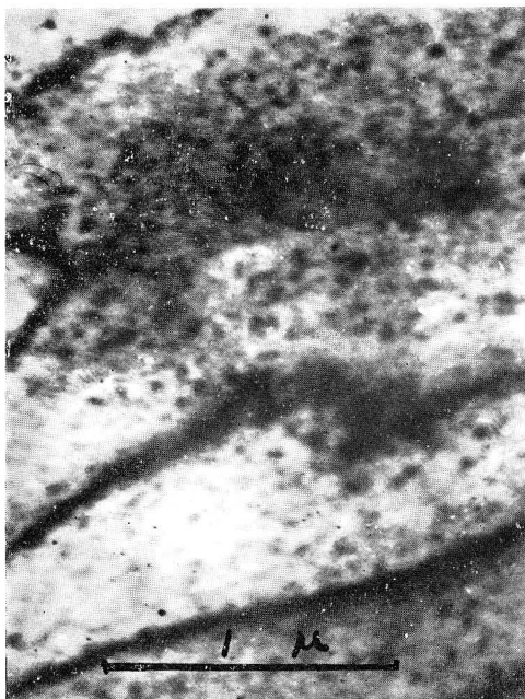
Photo. 25 Al-4% Cu alloy, W.Q., 40% rolled, aged for 4 days at 110°C. \times 35000
