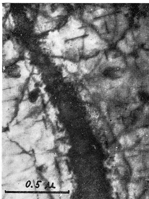
Photo. 27 Al-4% Cu alloy, W.Q., 5.0% elong., aged for 6 days at 160°C. ×54000
