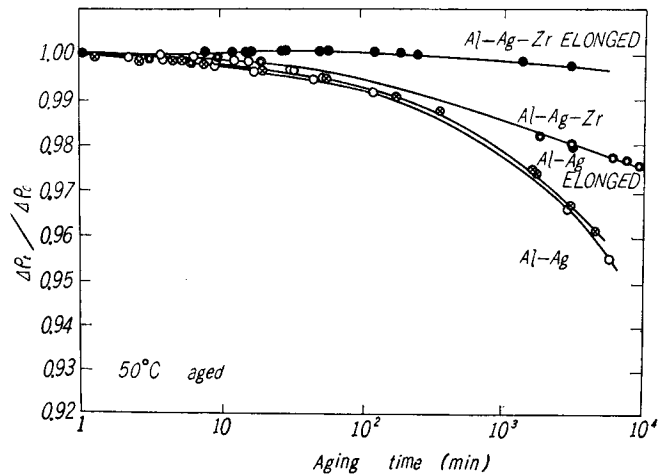
Fig. 10. Isothermal aging curves of resistivity at 50°C in undeformed or deformed binary and ternary Al-20% Ag alloys.
