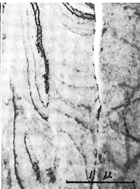
Photo. 32 Al-Cu-Zr alloy, W.Q., 70% rolled, aged for 70 days at 70°C. \times 30000
