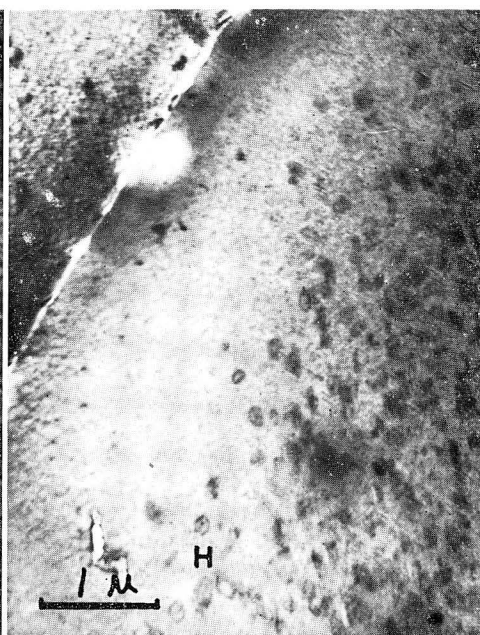
Photo. 48 Al-20% Ag alloy, W.Q., aged for 0.5 hrs at 200°C. \times 15000
