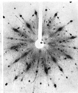
Photo. 18 Al-Cu-Zr alloy, W.Q., aged 12 hrs at 200°C.
