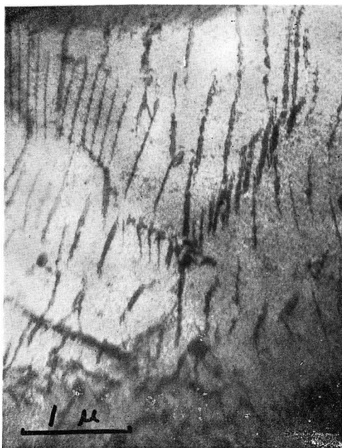
Photo. 45 Al-Ag-Zr alloy, W.Q., aged for 4 days at 110°C. \times 20000
