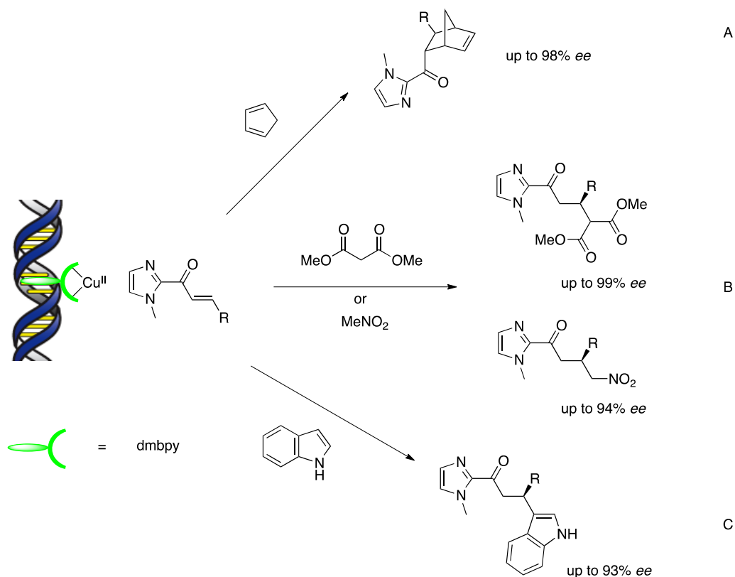
Scheme 4. Reaction scope of carbon-carbon bond forming reaction by DNA-based hybrid catalysts. (A) Diels–Alder reaction; (B) Michael addition; (C) Friedel–Crafts alkylation.
