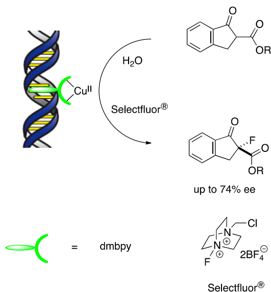
Scheme 5. Enantioselective C–F bond formation catalyzed by copper(II)-dmbpy-DNA.
