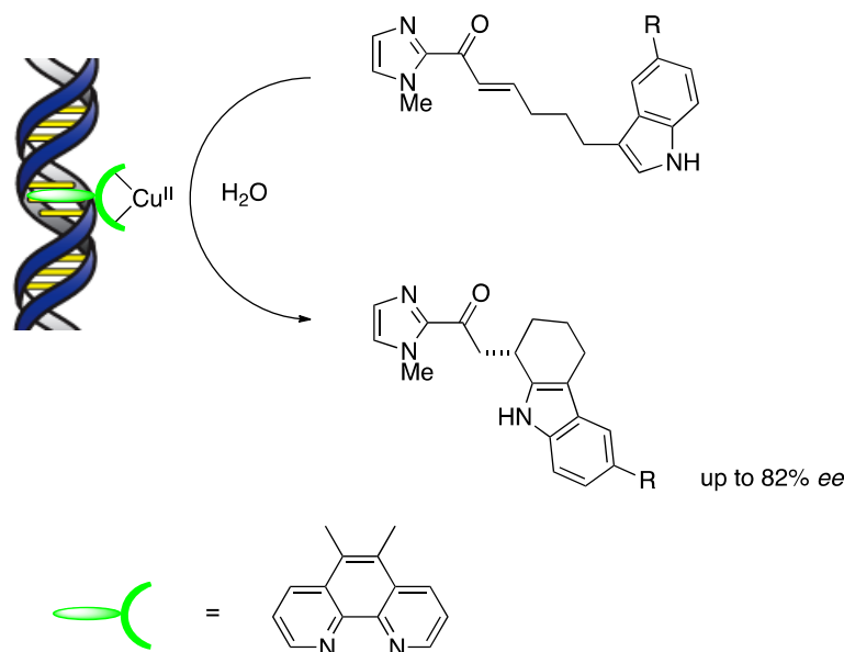
Scheme 8. Asymmetric intramolecular Friedel–Crafts alkylations with a DNA-based hybrid catalyst.
