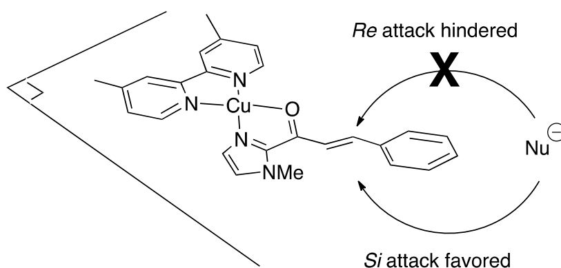
Scheme 9. Stereofacial selectivity of the attack of the nucleophile in the DNA-based catalytic asymmetric Diels–Alder and Michael reaction of \alpha,\beta -unsaturated 2-acyl imidazoles.
