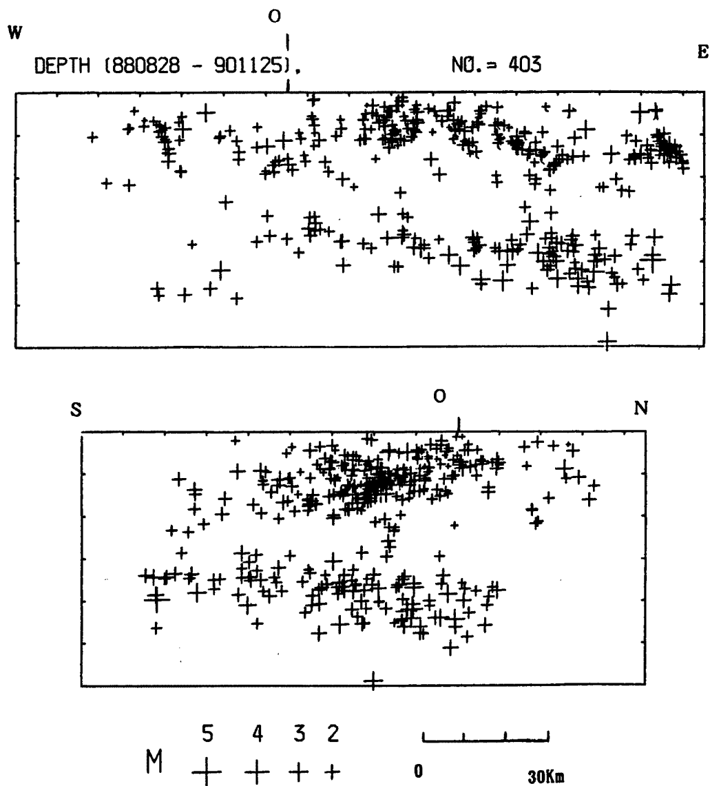
Fig. 8. Depth distribution of earthquakes determined by the new system. The symbol "0" shows the cross point of 134^{\circ} E and 34^{\circ} N lines.
