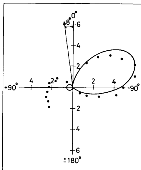
Fig. 3 Triple-differential cross section for 256.6 eV electron-impact ionization of helium in units of 10^{-3} a_0^2/\text{sr}^2 \text{ Ry} . The angle of observation for the faster electron \theta_f is 8^\circ and the energy of the slower electron E_s is 3 eV. Symbols are the same as in Fig. 1.
