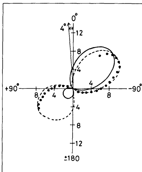
Fig. 1 Triple-differential cross section for 256.6 eV electron-impact ionization of helium in units of 10^{-3} a_0^2/\text{sr}^2 Ry . The angle of observation for the faster electron \theta_f is 4^\circ and the energy of the slower electron E_s is 3 eV. The solid curve is the present calculations. The dashed curve is the results calculated by Madison et al. The closed circles are the experimental data of Ehrhardt et al.
