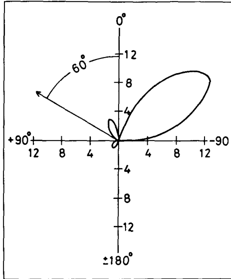
Fig. 4 Triple-differential cross section for 256.6 eV electron-impact ionization of helium in units of 10^{-8} a_0^2/sr^2 Ry . The angle of observaion for the faster electron \theta_f is 60^\circ and the energy of the slower electron E_s is 3 eV. The solid curve is the present calculation.
