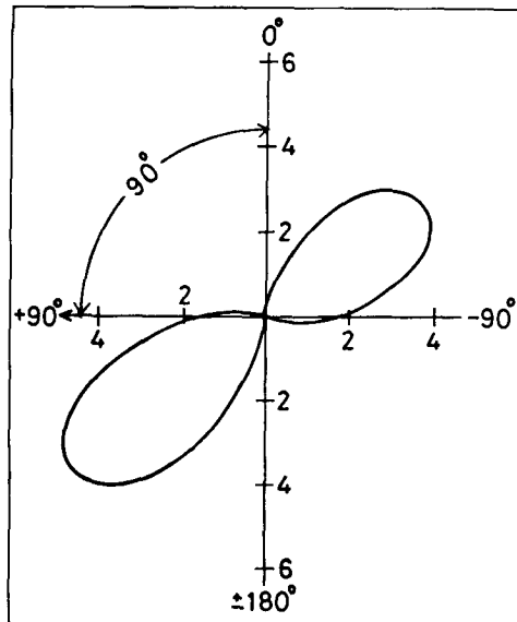
Fig. 5 Triple-differential cross section for 256.6 eV electron-impact ionization of helium in units of 10^{-8} a_0^2/sr^2 Ry . The angle of observation for the faster electron \theta_f is 90^\circ and the energy of the slower electron E_s is 3 eV. The solid curve is the present calculation.
