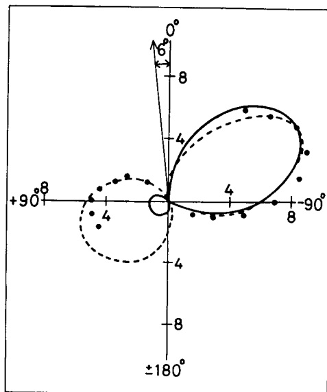
Fig. 2 Triple-differential cross section for 256.6 eV electron-impact ionization of helium in units of 10^{-3} a_0^2/\text{sr}^2 \text{ Ry} . The angle of observation for the faster electron \theta_f is 6^\circ and the energy of the slower electron E_s is 3 eV. Symbols are the same as in Fig. 1.
