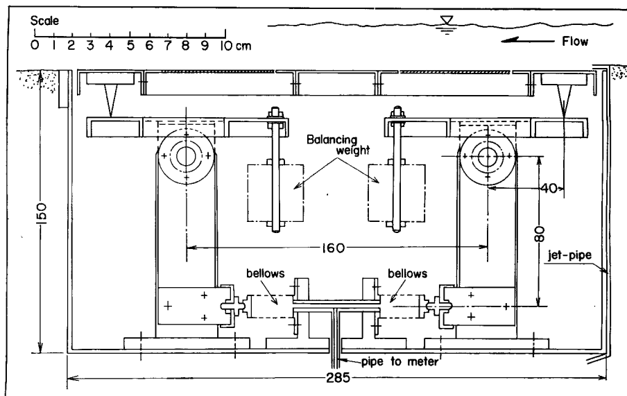
Fig. 14 Design of balance type measurement device.
