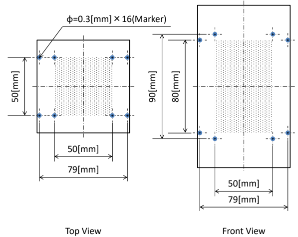
Fig. 8. Arrangement of voids in glass cuboid.
