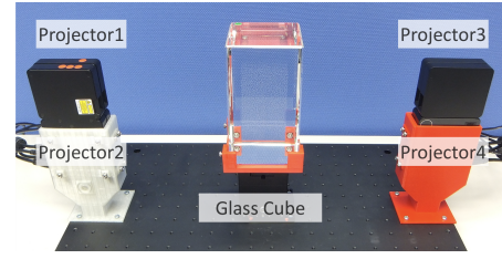
Fig. 11. Appearance of high-resolution display.
