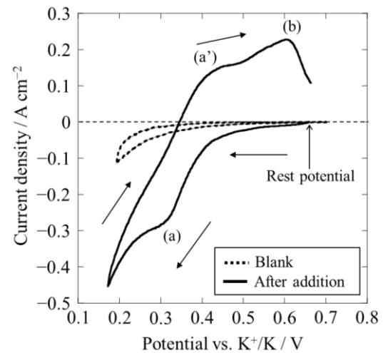
Fig. 3 Cyclic voltammograms for a Mo flag electrode in molten KF–KCl before and after the addition of \text{K}_2\text{TiF}_6 (0.10 mol%) and Ti sponge (0.033 mol%) at 923 K. Scan rate: 0.20 \text{ V s}^{-1} .
