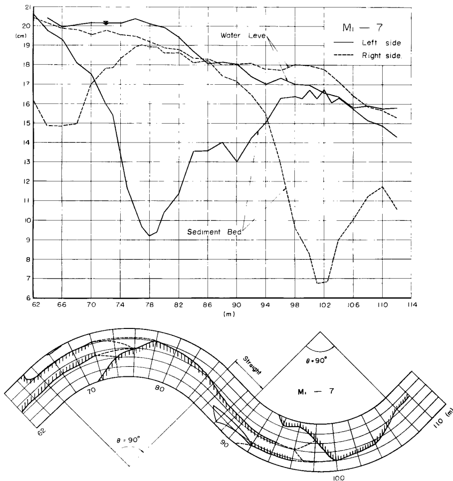
Fig. 12 (1) Profile of the water level and of the sediment bed along the side walls, and forms of the dunes. ( M_1 )
