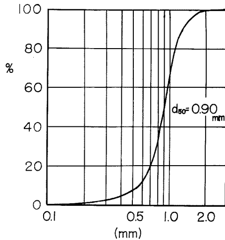
Fig. 2 Grain-size accumulation curve of used sand.
