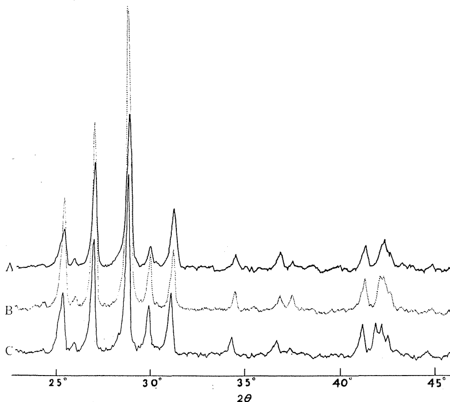
Fig. 5. Diffraction patterns of monazite from Nogizawa-mura, Japan. Cu-K \alpha (with Ni -filter), 35kV, 15mA. Scan speed 1° per minute, scaler 8, time constant 8, chart speed ½ inch per minute, slits 1°-0.006"-1°. A. Heated to ca 1950°C. B. Heated to ca 1800°C. C. Unheated.
