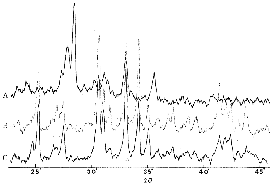
Fig. 1. Diffraction patterns of allanite from Anak-ub, Korea. Cu-Kα (with Ni -filter), 35 kV , 15 mA . Scan speed 1° per minute, scaler 4, time constant 8, chart speed ½ inch per minute, slits 1°-0.006"-1°. A. Heated to ca 1400°C. B. Heated at ca 800°C for two hours in the vacuum. C. Unheated.
