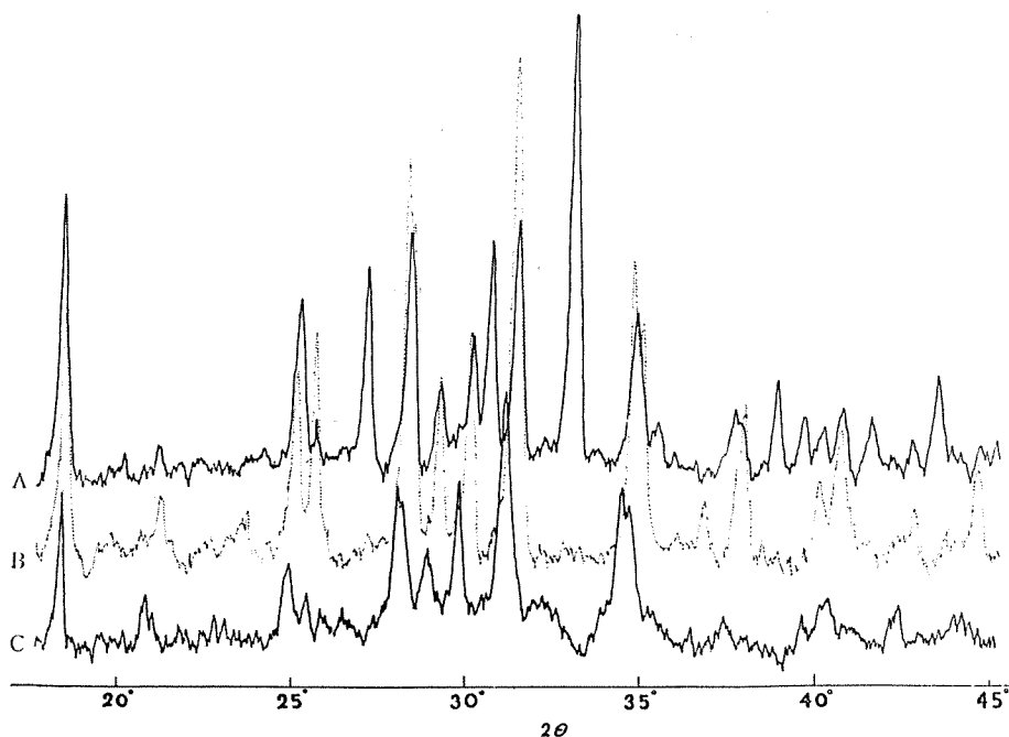
Fig. 2. Diffraction patterns of gadolinite from Arendal, Norway. Cu-K \alpha (with Ni-filter ), 35 kV , 15 mA . Scan speed 1° per minute, scaler 4, time constant 8, chart speed ½ inch per minute, slits 1°-0.006"-1°. A. Heated to ca 1500°C. B. Heated at ca 800°C for two hours in the vacuum. C. Unheated.
