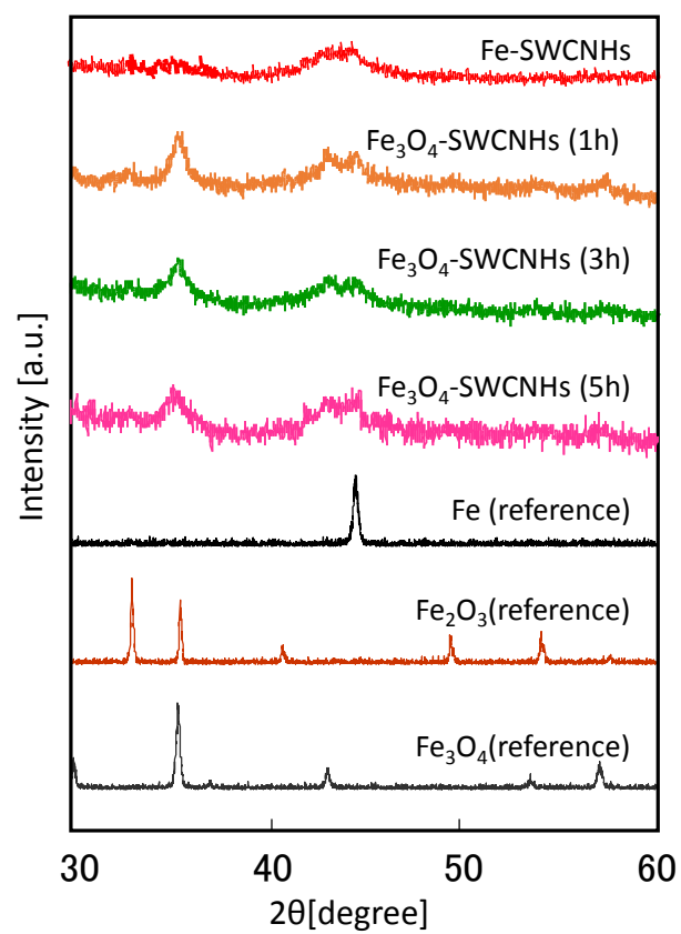
Fig. 2. XRD patterns of Fe-SWCNHs and \text{Fe}_3\text{O}_4 -SWCNHs prepared by varied ozone oxidation duration, 1, 3, and 5h together with XRD patterns of Fe, \text{Fe}_2\text{O}_3 and \text{Fe}_3\text{O}_4 for reference.
