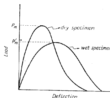
Fig. 3. Diagram of load-deflection curve.
