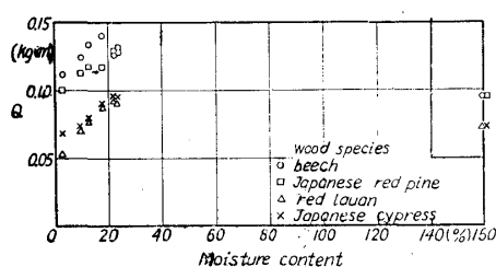
Fig. 2. Effect of moisture content on the energy consumption Q (in each wood specimen, expecting the average effect from other factors).
