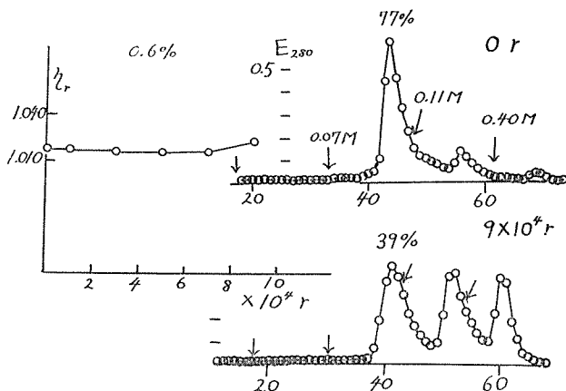
Fig. 1. The left diagram shows the relative viscosity of 0.6 per cent bovine plasma albumin solution ( 0.02 M sodium phosphate buffer pH 6.8) against dose of \gamma -rays having an intensity of 2.4 \times 10^5 r per hour. The right upper and lower diagram show column chromatogram of unirradiated and irradiated ( 9 \times 10^4 r) albumin. The abscissa and ordinate show tube numbers of fraction collector and extinction at 280 m\mu , respectively.
