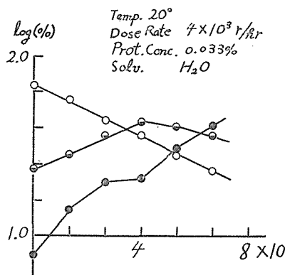
Fig. 4. Effect of \gamma -rays on chromatogram of bovine plasma albumin. ○, ◐ and ● showed three subfractions which were eluted with 0.07 M 0.11 M and 0.40 M sodium phosphate buffer pH 6.8, respectively. The ordinate and abscissa showed log (%) of three subfractions and dose of \gamma -rays, respectively. \gamma -ray irradiation was performed under the following conditions: solvent redistilled water, protein concentration 0.033 per cent, temperature 20°C, dose rate 4 \times 10^3 r per hour.
