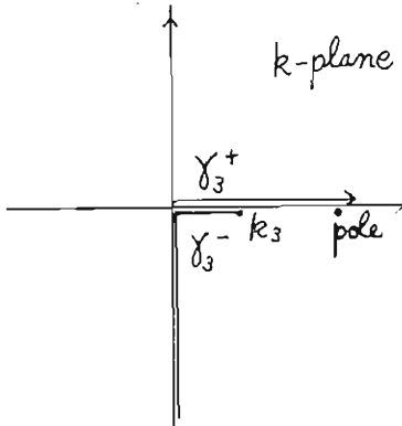
Fig. 2 Branch line and residues in k -plane.
