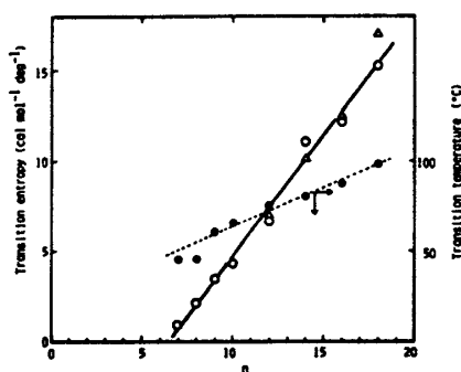
図9. Transition entropy and transition temperature vs. the number of carbon atoms ( n ). The values (O) and (Δ) were obtained from the peaks during heating and cooling scans, respectively.
