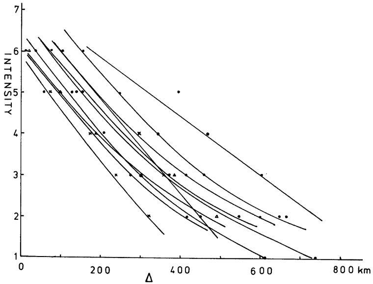
Fig. 1. Relations between seismic intensity and distance from seismic fault.
