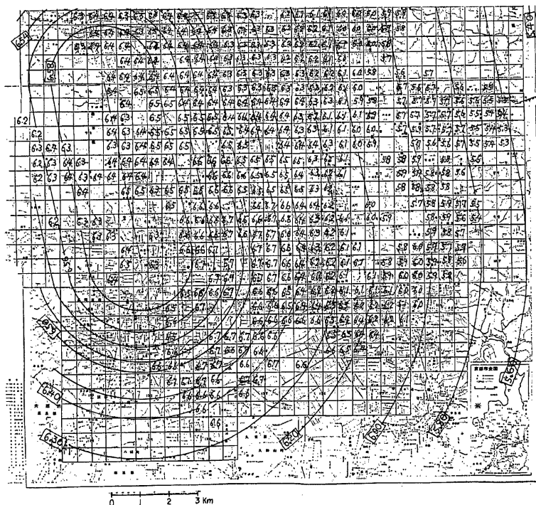
Fig. 5. Pattern of the seismic intensity at the southward of Kyoto in the Katagihara Earthquake ( M=6.5 ). It shows the intensity at the standard ground, for instance \underline{6.30} .
