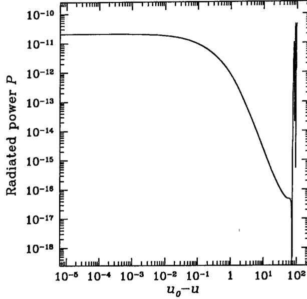
Figure 3.14: Plots of the radiated power P for globally naked case (a) at R = 100 . The horizontal axis is the out-going null coordinate u . At the Cauchy horizon, this coordinate has the value u_0 .
