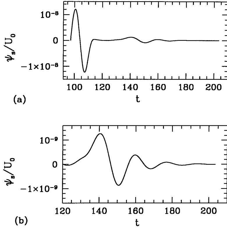
Figure 3.13: Plots of \psi_s for the black hole case (c) at R = 100 . In (a) the left-hand side oscillation originates from the initial ingoing wave. After this oscillation, the damped oscillation dominate, as depicted in (b).
