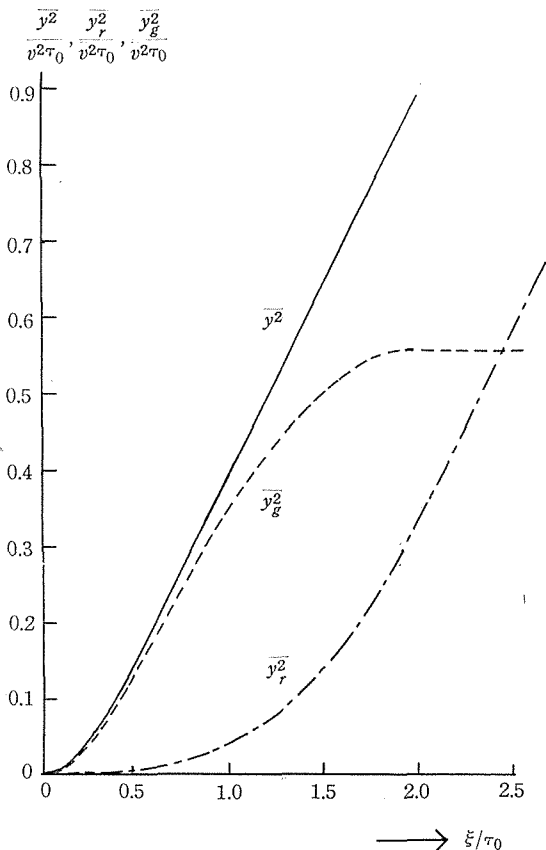
Fig. 4. Graphical illustration of \bar{y}^2(\xi) , \bar{y}_r^2(\xi) and \bar{y}_g^2(\xi) .
