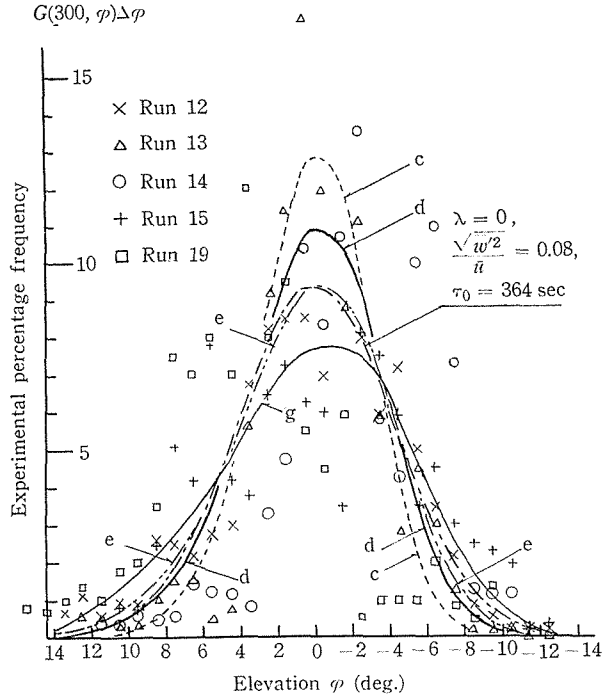
Fig. 7. Graphical illustration of theoretical values of flux G(300, \varphi)\Delta\varphi in case of \Delta\varphi = 1.745 \times 10^{-2} rad and Q=100 and the experimental percentage frequency of particles captured. Theoretical curves indicated as c , d , e and g correspond to those in Fig. 6.
