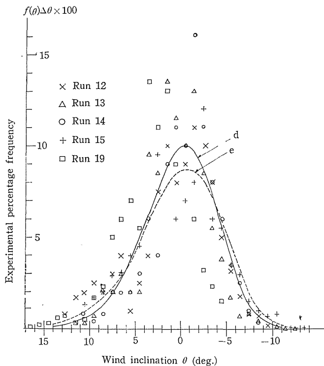
Fig. 8. Graphical illustration of theoretical values of wind inclination frequency f(\theta)\Delta\theta in the case of \Delta\beta = 1.745 \times 10^{-2} rad and the values of \lambda and \sqrt{\overline{w^2}}/\bar{u} identical with those in the case of d and e in Figs. 6 and 7, and the experimental percentage frequency of wind inclination corresponding to the experimental results of particle elevation in Fig. 7.
