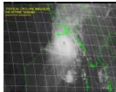
Fig.1 Satellite image of cyclone “Sidr” by Indian Meteorological Department
