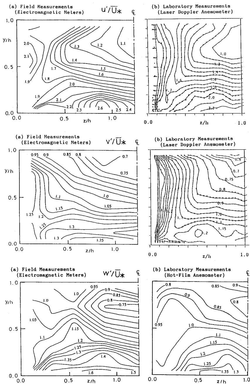
Figure 16 All three components of turbulence intensity, u' , v' and w' , for (a) field channel and (b) laboratory flume.
