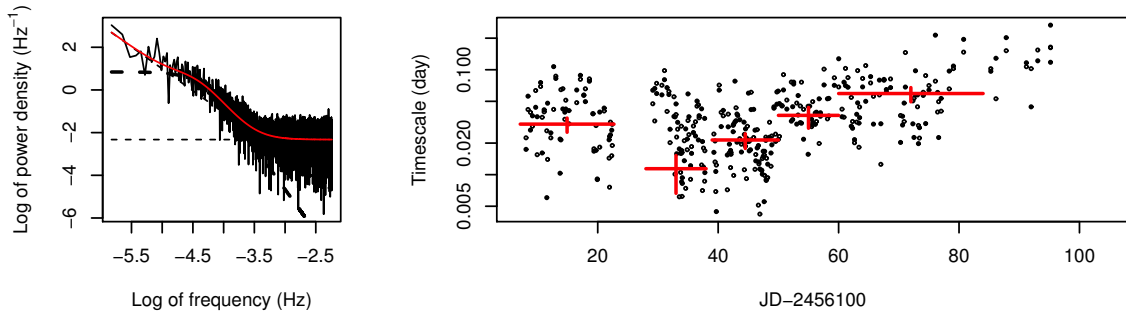
Figure 3. Example of calculated power spectrum density (left panel) and time series of variation timescales (right panel). In the left panel, the epoch of the light curve used in calculating the power is from JD 2456107 to 2456122. Red line shows the best-fit function of Equation (1), and dotted lines are each term of the best-fit function. In the right panel, filled and open circles are shown as doubling timescales in rise and decay phases of micro-variation events. Red points correspond to timescales estimated from the best-fit break frequencies of the power spectrum densities (PSDs) calculated for each epoch of the light curve.
