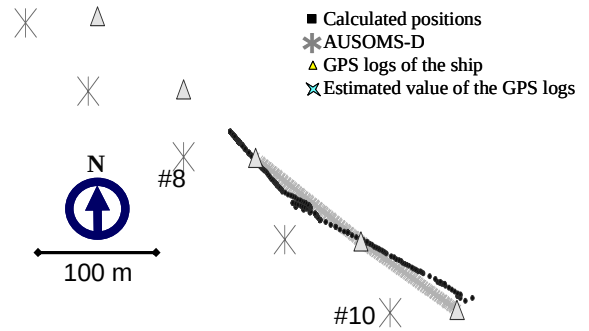
Fig. 10. Result of the localization of the sound source of the artificial dugong calls.
