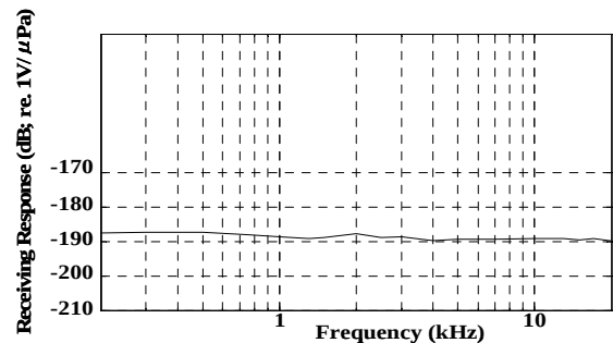
Fig. 4. Frequency characteristics of the hydrophone
