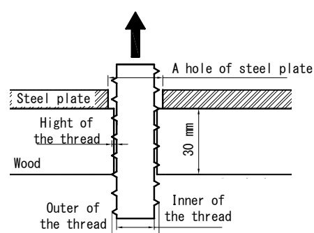
Fig. 1 Outline of test of pull-out screw
