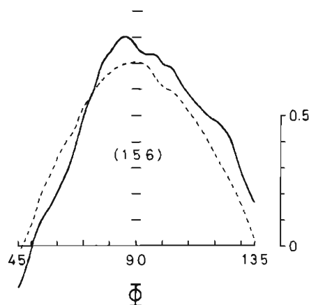
Fig. 40. Crosscorrelation for the earthquakes in Fig. 39. (Regions 4, 5, 6, 7)
