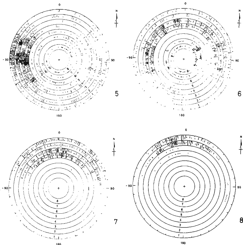
Fig. 33. Push-Pull distribution of the initial motions of P waves, setting the epicenters as origins (cross). Open circle: Push, Solid circle: Pull.
