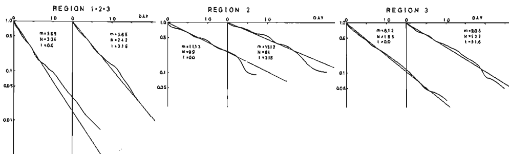
Fig. 30. Cumulative distribution of time intervals between adjacent earthquakes. N , m and l are the number of earthquakes, the number of earthquakes per unit time and the filtered time interval in the text respectively.
