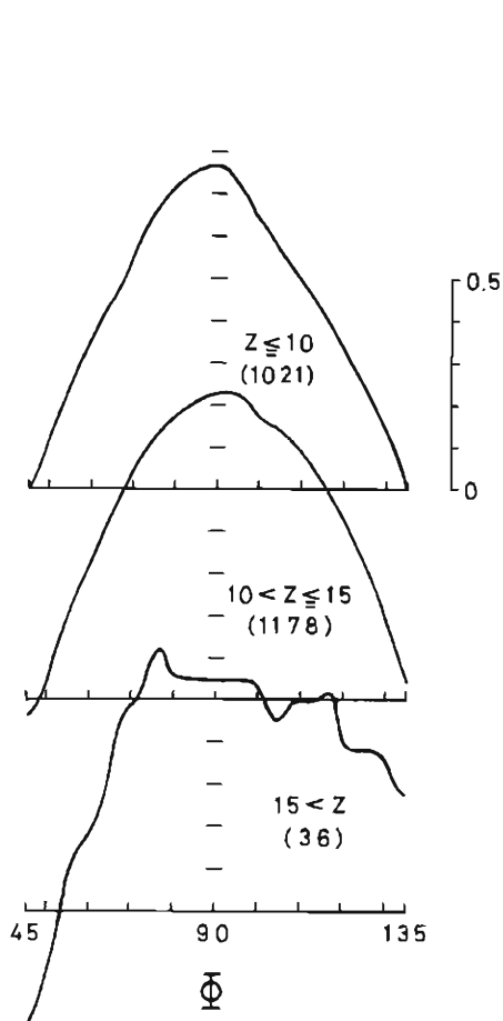
Fig. 38. Crosscorrelation relating to focal depth. (Regions 5, 6, 7)
