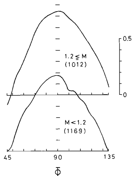
Fig. 36. Crosscorrelation relating to magnitude. Number of data is shown in parentheses. (Regions 4, 5, 6, 7)
