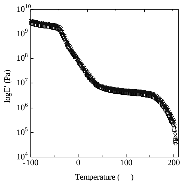
Figure 4-7. Storage modulus ( E' ) as functions of temperature for the WB 2K-PU films at different TAM: (○) 1 h, (□) 4 h and (×) 8 h.
