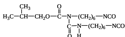
HDI Allophanate
