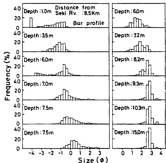
Fig. 17 Some examples of grain size distribution of bottom sediment, July 25, 1972.
