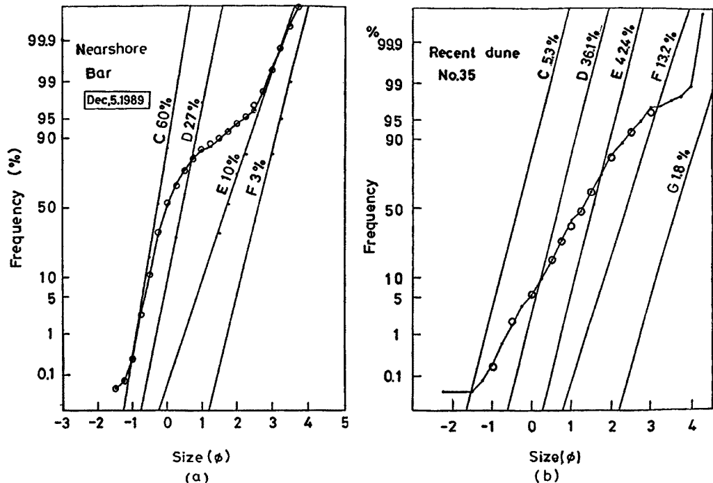
Fig. 21 Cumulative probability curve and constituent subpopulations derived by partitioning from the curve. Circles are the cumulative plots constructed from the partitioned constituent subpopulations.
