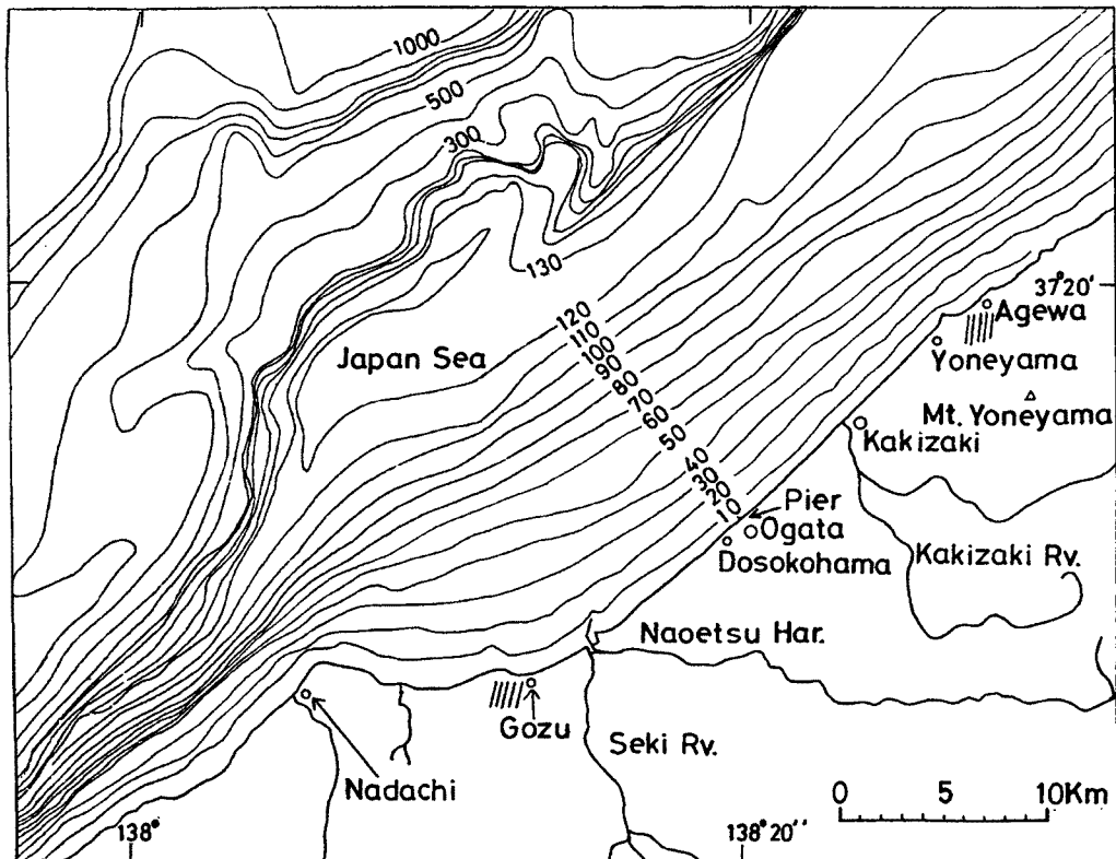
Fig. 3 Bottom topography of Ogata coast.
