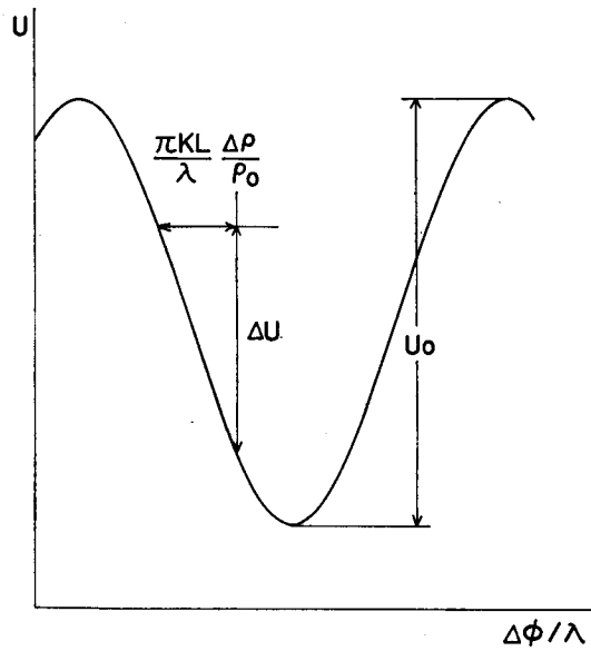
Fig. 3. Interference Curve.
