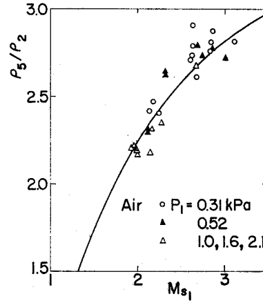
Fig. 16. Reflected Shock Density Ratio \rho_{s2} in Air.
