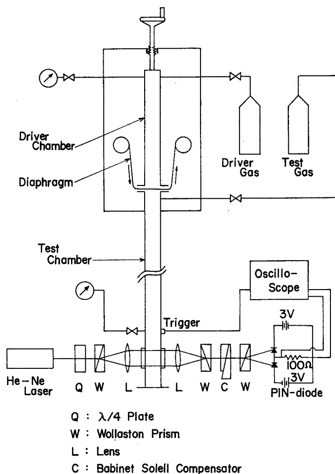
Fig. 4. Experimental Apparatus.
