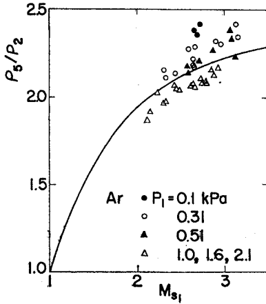
Fig. 15. Reflected Shock Density Ratio \rho_{s2} in Ar.
