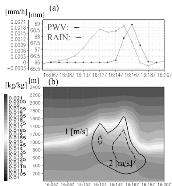
Figure 1. (a) Time variation of PWV and Rain at a certain point in NHM and (b) Time-height cross section of water vapor mixing ratio (shade) and vertical wind velocity (contour) at the same point in NHM.
