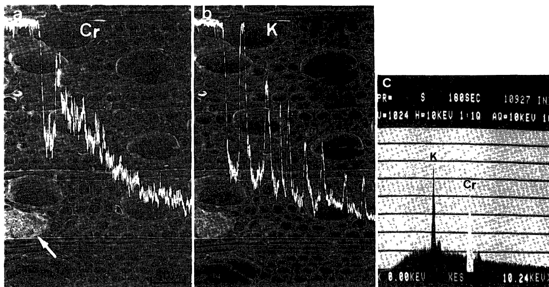
Fig. 6. Line scans of Cr-K \alpha and K-K \alpha X-ray and their X-ray spectrum of Hōnoki which was penetrated with the K 2 Cr 2 O 7 solution. a , b : Cross section at the height of 9.5 mm in longitudinal capillary rise for 4 hours. White arrow shows a deposition of K 2 Cr 2 O 7 in the vessel lumen. c : Energy dispersive X-ray spectrum on the scanning line in a .
