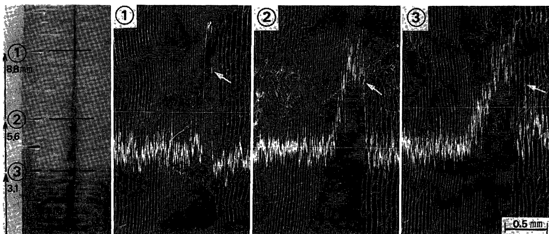
Fig. 4. Change of lateral distribution of chromium with the height from the base of the Ezomatsu specimen which was penetrated with the K_2Cr_2O_7 solution to the longitudinal direction for 4 hours. Note; a narrow and sharp curve (white arrow in ①) was drawn near the penetration front, but the slope of the curves gradually moderated and spreaded to the radial direction at the positions near the base (② and ③).
