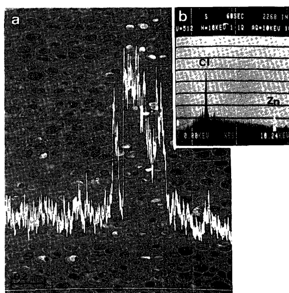
Fig. 8. Line scan of Zn-K \alpha X-ray of the cross section at the height of 18 mm from the base of Buna which was penetrated with the \text{ZnCl}_2 solution for 4 hours ( a ) and the X-ray spectrum on the scanning line in a ( b ).
