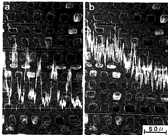
Fig. 1. Line analysis of Cr-K \alpha X-ray on the cross-sectional surface of Ezomatsu which was penetrated with the K 2 Cr 2 O 7 solution. a : Line scan along the center of a radial file of cells. b : Line scan on the double cell wall between the two radial files of tracheids.
