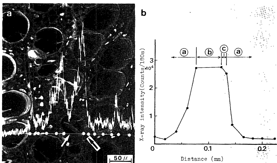
Fig. 3. SEM-EDXA of Cr- K_{\alpha} X-ray of Buna which was penetrated with the K_2Cr_2O_7 solution. a: Cross-sectional view at the penetration height of 9.9 mm and line-scan to the tangential direction. b: Point analysis at the positions with white points on the line in a. (a); Region of ionic diffusion through the cell wall. (b); Initially penetrated vessel which was indicated with the white arrow in a. (c); Lateral liquid-flow from the vessel to a adjacent cell which was indicated with the black in a.
