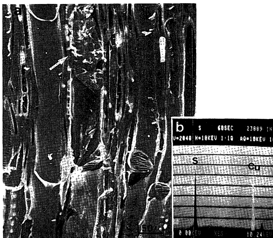
Fig. 7. A SEM micrograph of Buna showing the \text{CuSO}_4 precipitation in the vessel lumen (white arrow in a ) and the X-ray spectrum of the precipitate ( b ).
