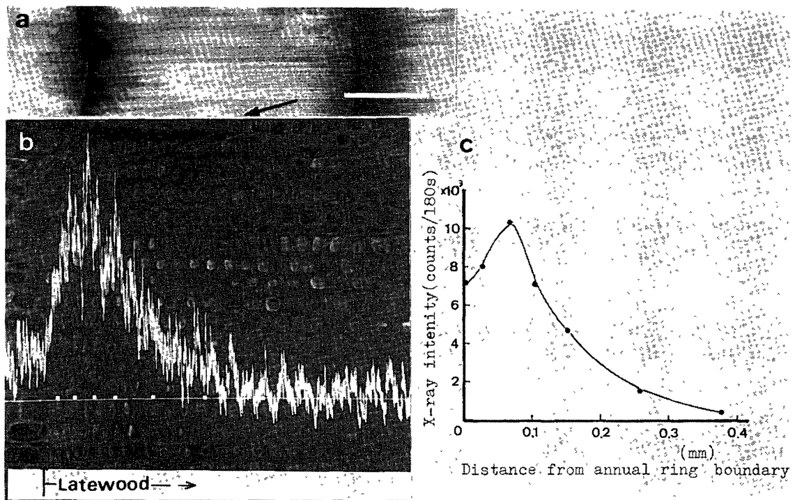
Fig. 2. Line and point analyses of Cr-K \alpha X-ray on the double cell walls along the radial file of cells of Ezomatsu which was penetrated with the K 2 Cr 2 O 7 solution for 4 hours. a : LM micrograph of cross section at the penetration height of 5.5 mm. b : Line scan on the white line in a . White points on the line show the position of point analysis. c : point analysis at the various positions on the line in b .
