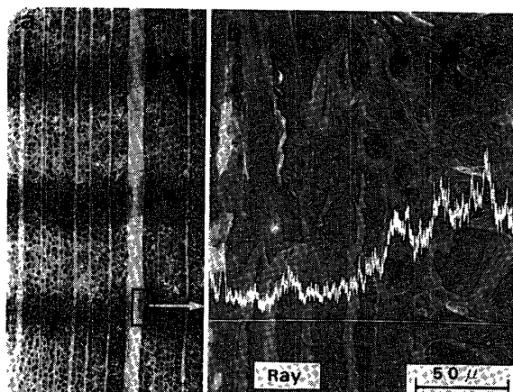
Fig. 5. Distribution of chromium across the multiseriate ray of Buna. a : LM image of cross-section at the penetration height of 9.9 mm in longitudinal capillary rise for 4 hours. b : Line scan of Cr-K \alpha X-ray across the ray tissue.
