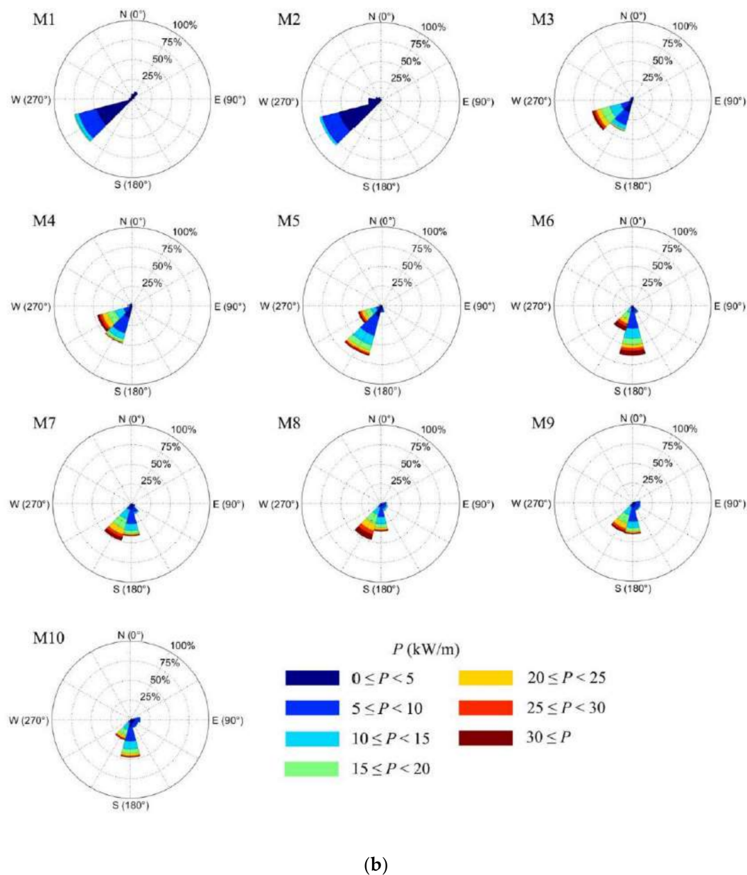
Figure 12. (a) Wave power roses at locations M1 to M10 under the “present” climate. (b) Wave power roses at locations M1 to M10 under the “future” climate.
