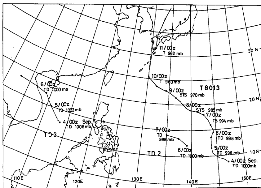
Fig. 1. Tracks of Typhoon 8013 (ORCHID) and other two tropical depressions. (●-00Z, ○-12Z)
