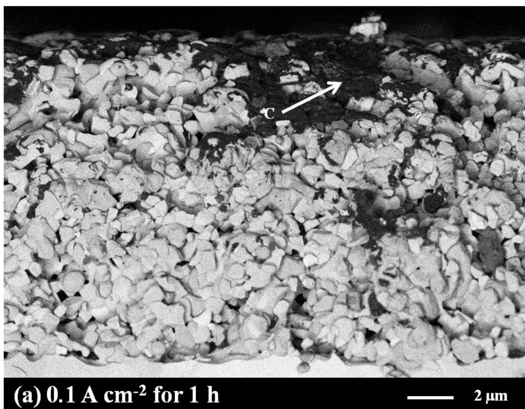
Figure 4.8. Backscattered electron images for the Ni-YSZ anode layer after removing carbon by discharge at (a) 0.1 \text{ A cm}^{-2} in 10% \text{H}_2 –90% He for 1 h.
