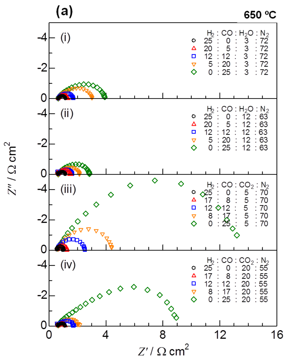
Figure 3.3. AC impedance spectra for the (a) electrolyte-cells with a supply of \text{H}_2 -CO- \text{H}_2\text{O} (or \text{CO}_2 ) mixture at 650 °C. The impedances were measured between the anode, and reference electrode for the electrolyte-supported cell and between the anode and cathode for anode-supported cell.
