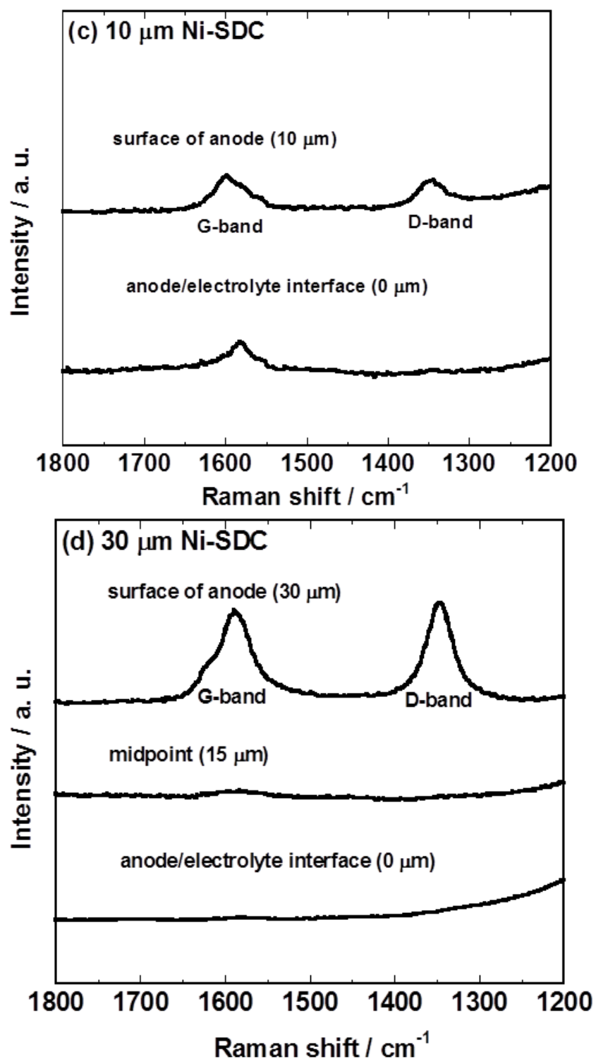
Figure 1.7. Raman spectra of anode along the electrode thickness direction for (c) 10-μm and (d) 30-μm thick Ni-SDC after discharge at 0.2 A cm -2 with a supply of CH 4 -H 2 O-N 2 mixture (S/C = 0.1) at 1000 °C.
