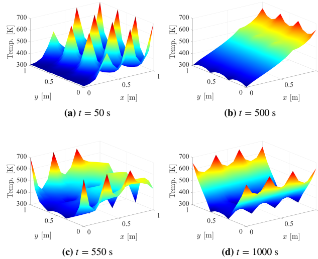
Figure 4 Temperature distributions at different time t
