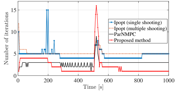
Figure 6 Time histories of numbers of iterations
