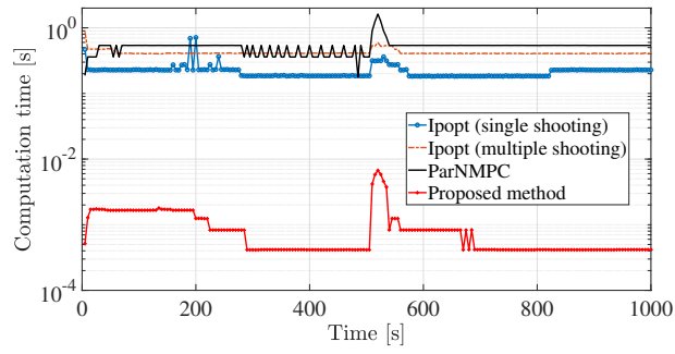
Figure 7 Time histories of computation times per time step
