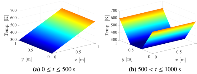
Figure 3 Temperature distribution references at different time periods
