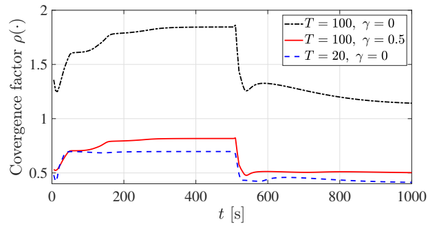
Figure 8 Time histories of convergence factors of SGS under different settings
