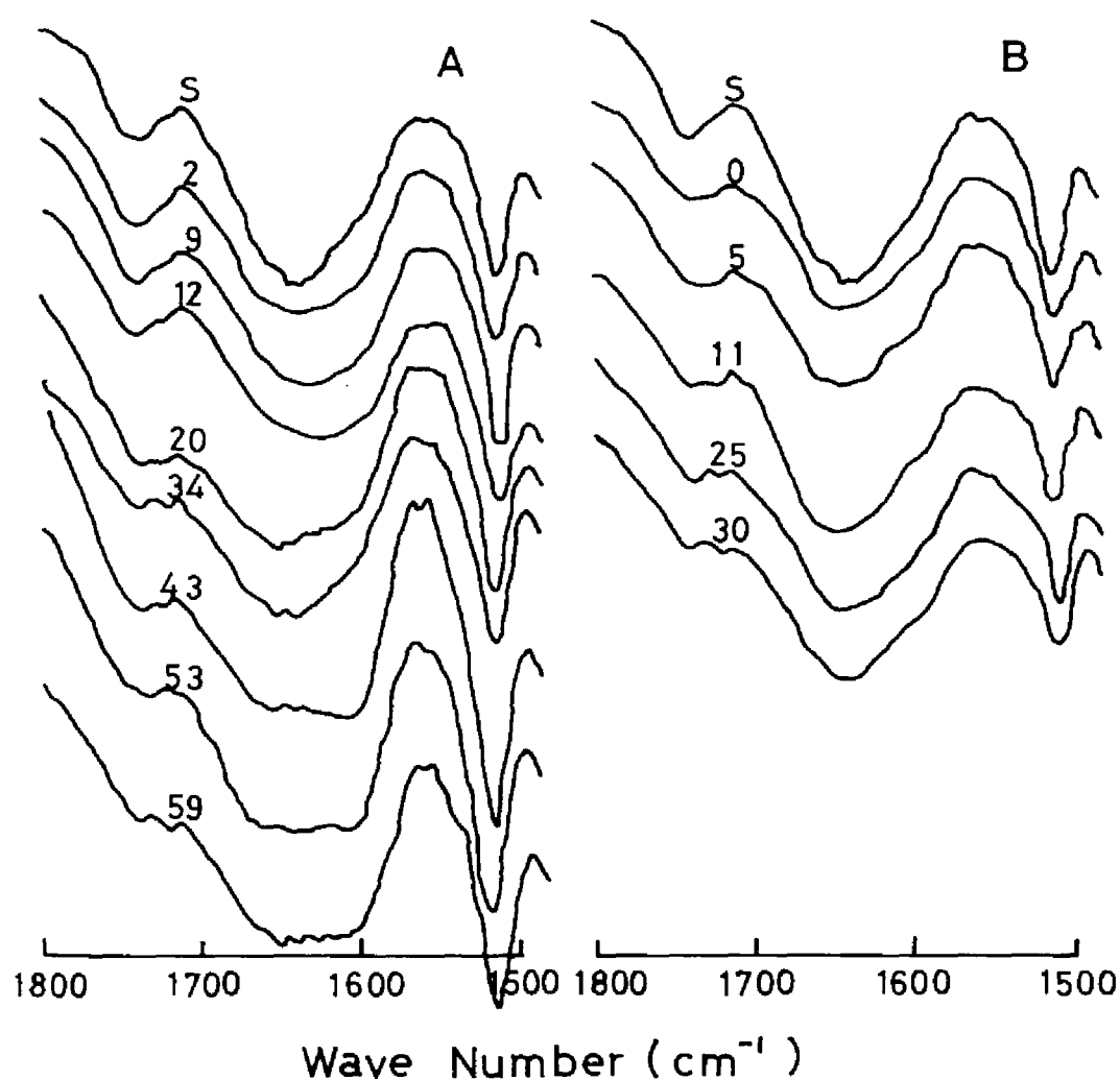
Fig. 20. Infrared spectra of wood of Cryptomeria japonica exposed to Tyromyces palustris (A) and Coriolus versicolor (B) in the 1800-1500 cm -1 region. S: Sound wood, Figure on spectra: % weight loss in wood block.
