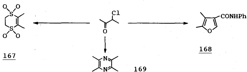
Scheme 67
