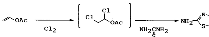
Scheme 17
