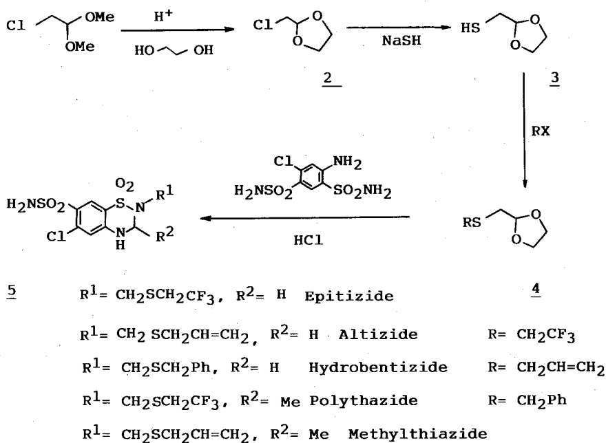
Scheme 8
