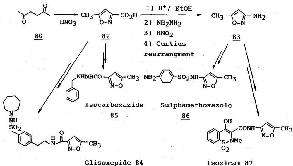
Scheme 38
