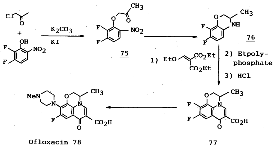
Scheme 35
