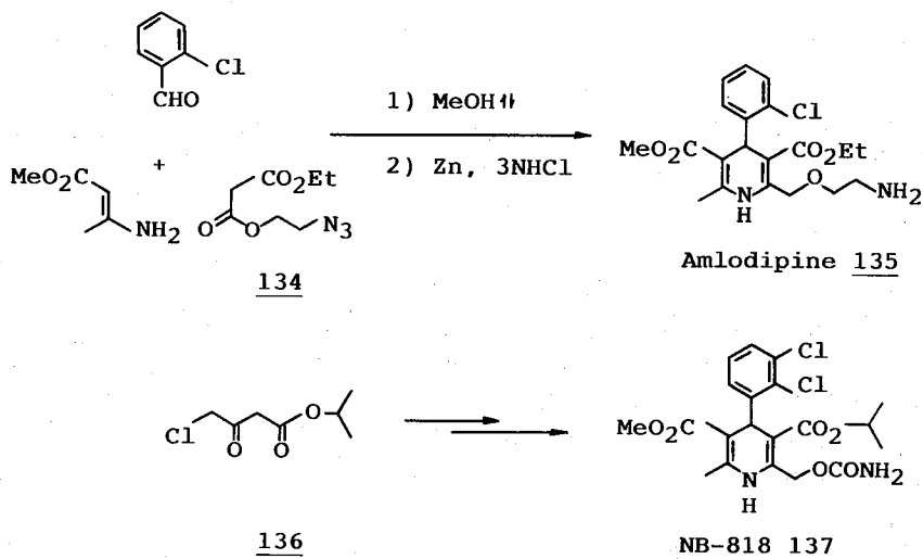
Scheme 57
