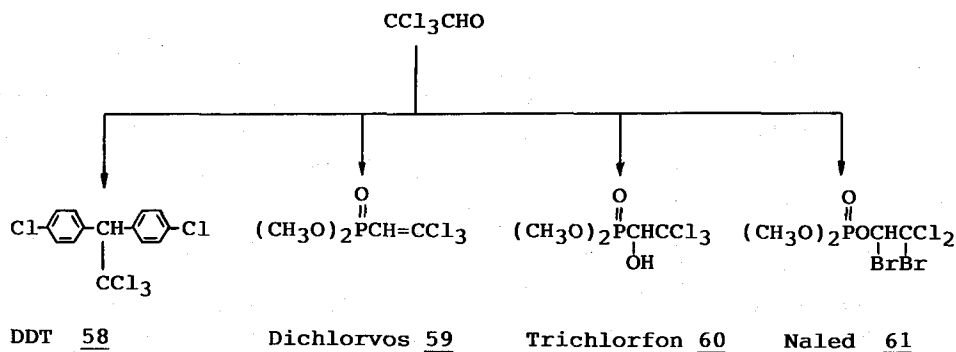
Scheme 27
