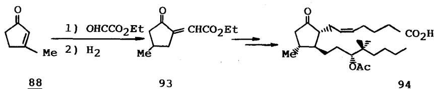
Scheme 39
