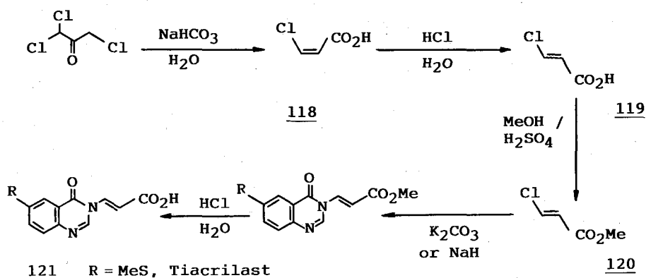
Scheme 51
