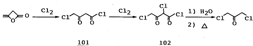
Scheme 43
