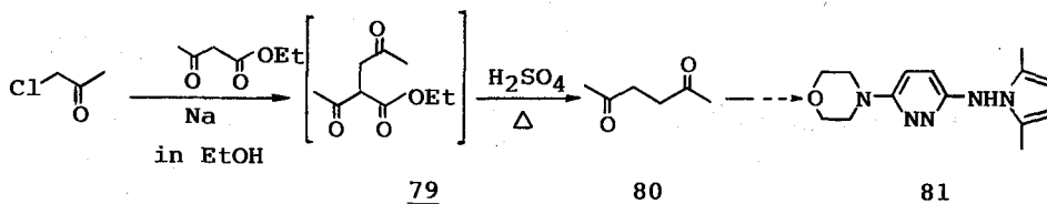
Scheme 36
