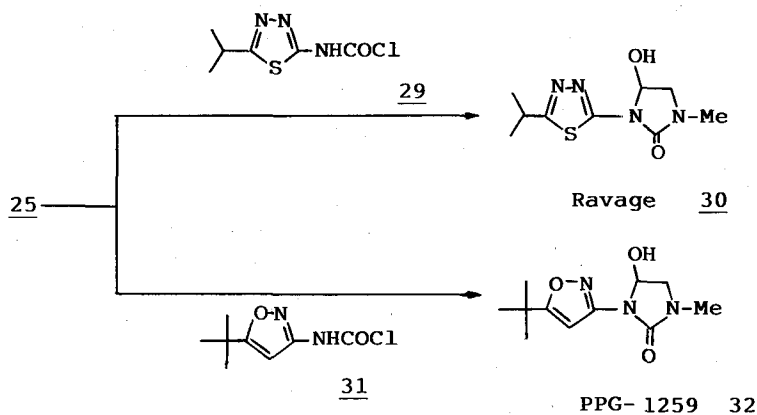
Scheme 16
