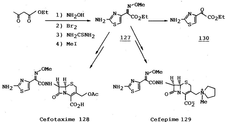
Scheme 55
