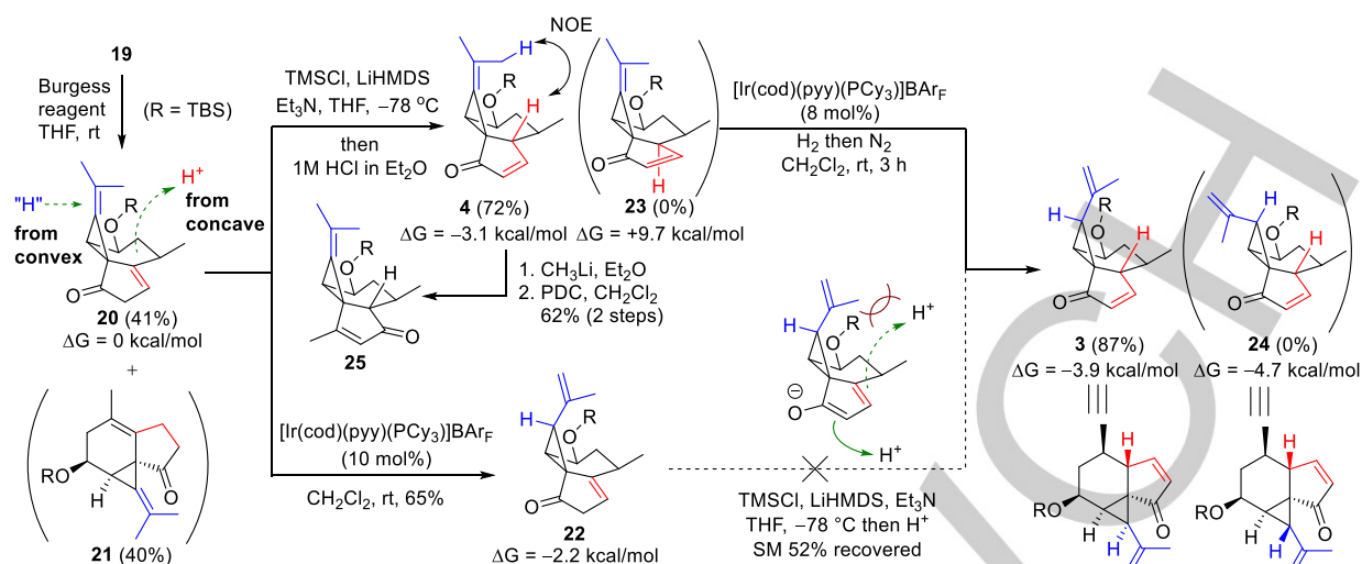
Scheme 3. Stereoselectivity of diastereoselective double-bond isomerization and relative thermodynamic stabilities of intermediates calculated by Spartan 18 at the \omega B97X-D/6-31G* level of theory.
