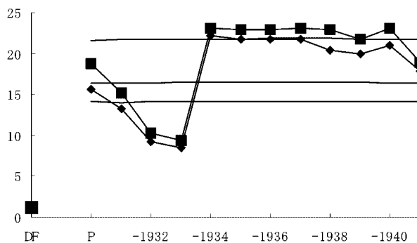
Figure 6.2 Interval \Psi and \tau^2 ratios (A model).
