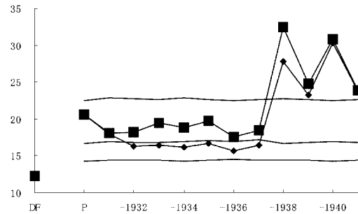
Figure 3.2 Interval \Psi and \tau^2 ratios (A model).
