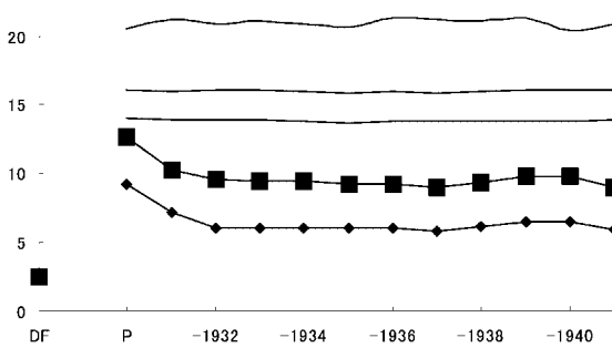
Figure 4.2 Interval \Psi and \tau^2 ratios (A model).
