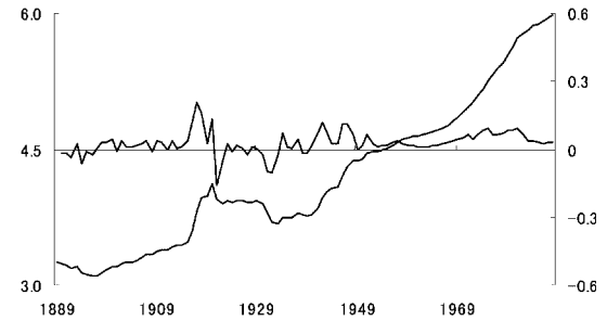
Figure 4.1 Natural log of GNP deflator and the first difference.
