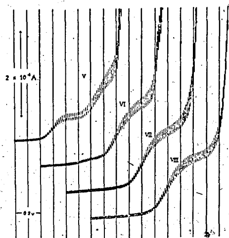
Fig. 7—Polarograms of 11.4 \times 10^{-4} M. 'pyrethrins' II reduced at different pH values: V (pH=5.67), VI (pH=6.73), VII (pH=7.64), VIII (pH=9.02). Each polarogram begins at -1.00 v.
