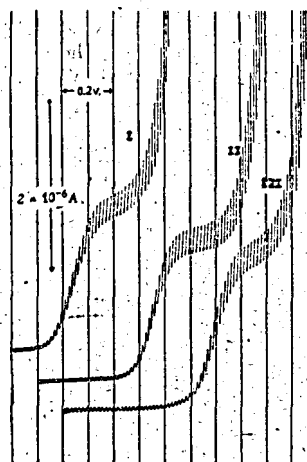
Fig. 2—Influence of indifferent salt on reduction wave of mixture of 'pyrethrins' I and II (1:1): I ( \text{M}/5 \text{ KI} ), II ( \text{M}/5 (\text{CH}_3)_4\text{NBr} ), III ( \text{M}/5 \text{ NaCl} ). Each polarogram begins at -0.80 \text{ v} .
