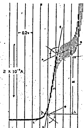
Fig. 11 Method of measuring wave height.
