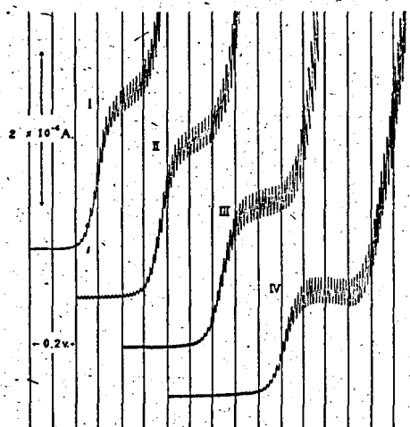
Fig. 3—Polarograms of 12.4 \times 10^{-4} \text{ M.} 'pyrethrins' I reduced at different pH values: I ( \text{pH}=1.49 ), II ( \text{pH}=2.56 ), III ( \text{pH}=3.63 ), IV ( \text{pH}=4.99 ). Each polarogram begins at -0.80 \text{ v} .
