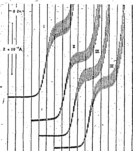
Fig. 1—Polarograms of standard matters: I \alpha -dl-trans-allethrin ( 20 \times 10^{-4} \text{ M.} ), II 'pyrethrins' II ( 20 \times 10^{-4} \text{ M.} ), III mixture of 'pyrethrins' I and II ( 20 \times 10^{-4} \text{ M.} ), IV 'pyrethrins' I ( 20 \times 10^{-4} \text{ M.} ). Each polarogram begins at -0.80 \text{ v} .
