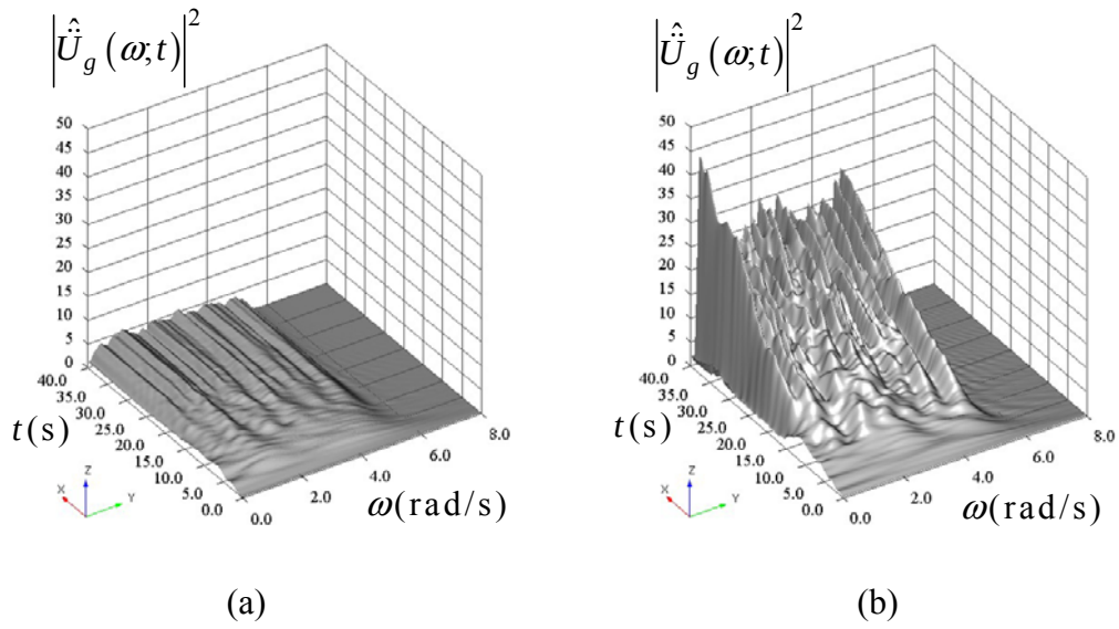
Fig.15 Average value of SFAS of 100 ground motions truncated at continuously increasing time: (a) non-stationary input, (b) stationary input
