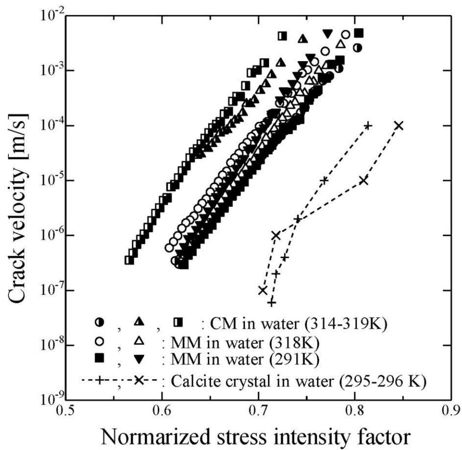
Figure 9. Relationship between crack velocity and stress intensity factor normalized by fracture toughness for marble and calcite crystal. “×” and “+” are the relationships obtained by Røyne et al. (2011) and Rostom et al. (2012), respectively.
