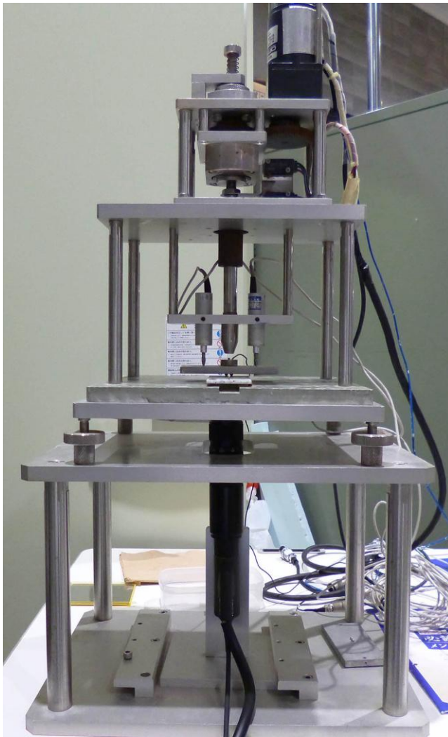
Figure A-1. Photo of apparatus of fracture toughness measurement by DT-CDR test.
