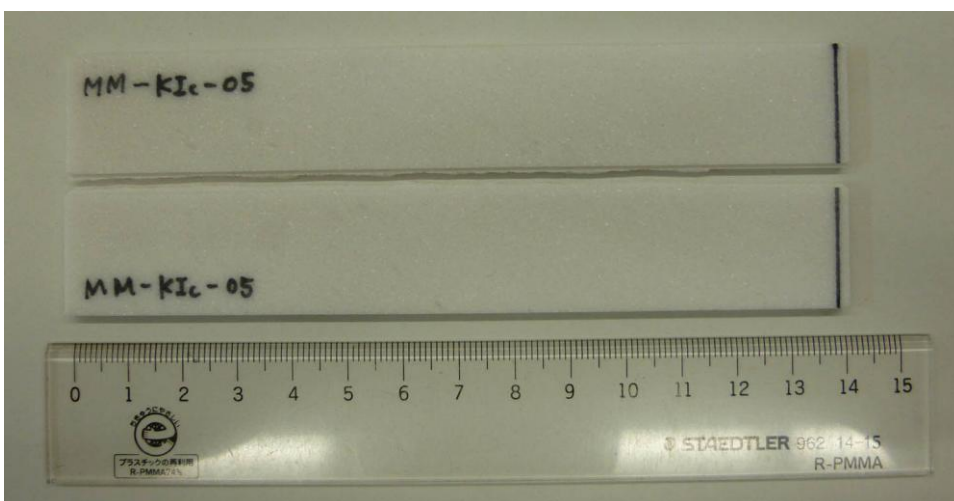
Figure A-2. Photo of DT specimen of Macedonian marble used in fracture toughness measurement
