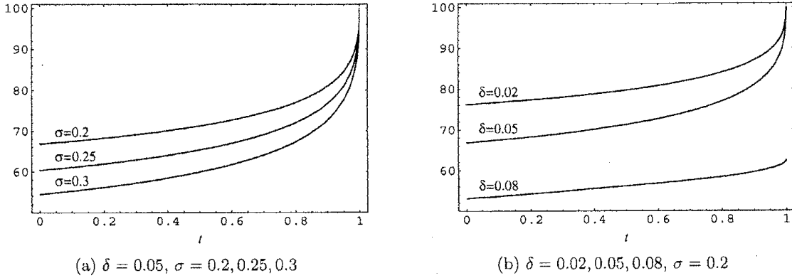
Figure 6: Early exercise boundaries of put options ( K = 100 , T = 1.0 , r = 0.05 )
