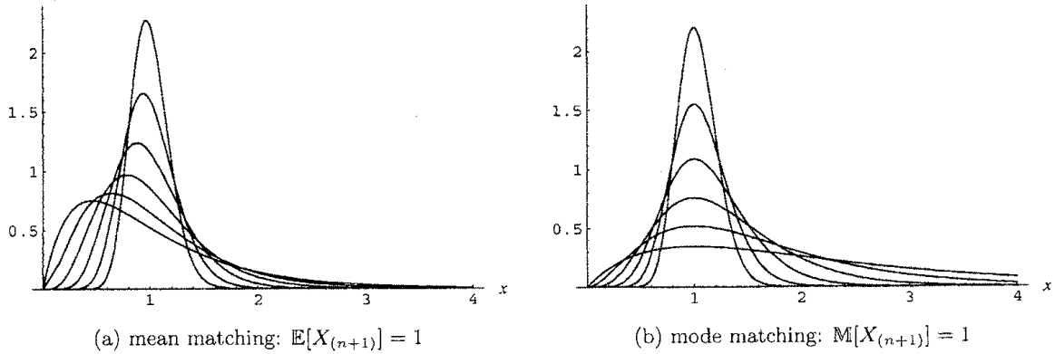
Figure 2: Probability density functions of the order statistic ( n = m = 1, 2, 4, 8, 16, 32 )
