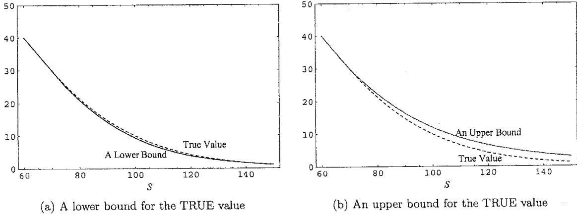
Figure 3: Lower and upper bounds ( T = 1.0 , S = 100 , K = 100 , r = 0.05 , \sigma = 0.3 , \delta = 0 )
