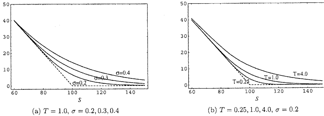
Figure 7: Values of put options ( K = 100 , t = 0 , r = 0.05 , \delta = 0.02 )
