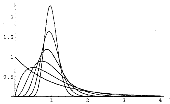
Figure 1: n -stage Erlangian probability density functions ( n = 1, 2, 4, 8, 16, 32 )
