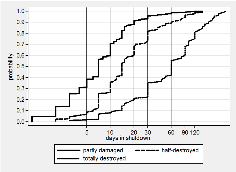
Figure 6. Cumulative Distribution of Plants and Period of Operational Shutdown
